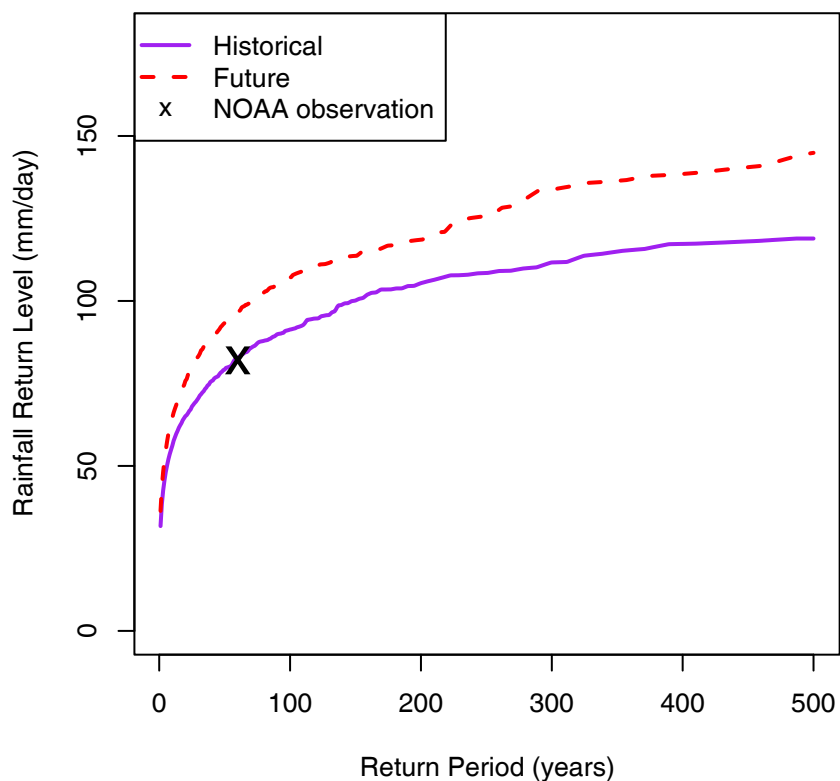
(c) Edinburgh: Rainfall return level curve
