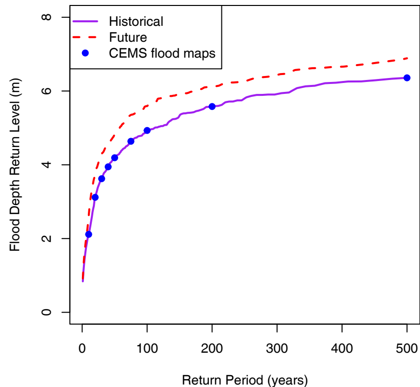
(b) Gothenburg: Flood depth return level curve
