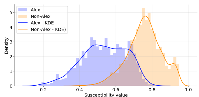
Figure 12. Kernel density estimates (KDE) distributions of susceptibility values at the locations of Alex (blue) and non-Alex (orange) landslides on the WoSAL map.
