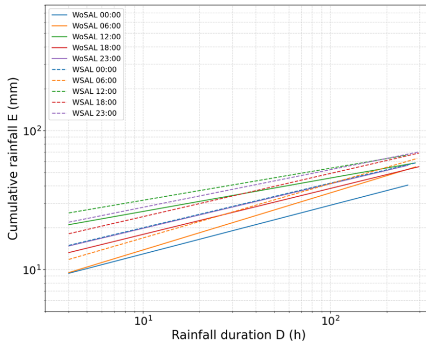
Figure A4. ED thresholds calculated with a 5 % quantile regression, depending on the assumed hour of occurrence of landslides (00:00, 06:00, 12:00, 18:00, and 23:00). Solid lines correspond to WoSAL thresholds, while dashed lines indicate WSAL thresholds.
