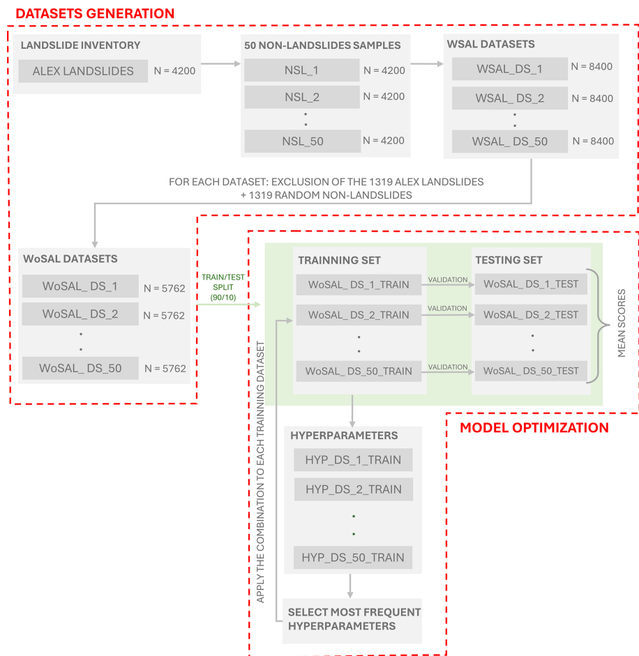
Figure 5. Workflow of dataset generation and RF optimization procedures.
