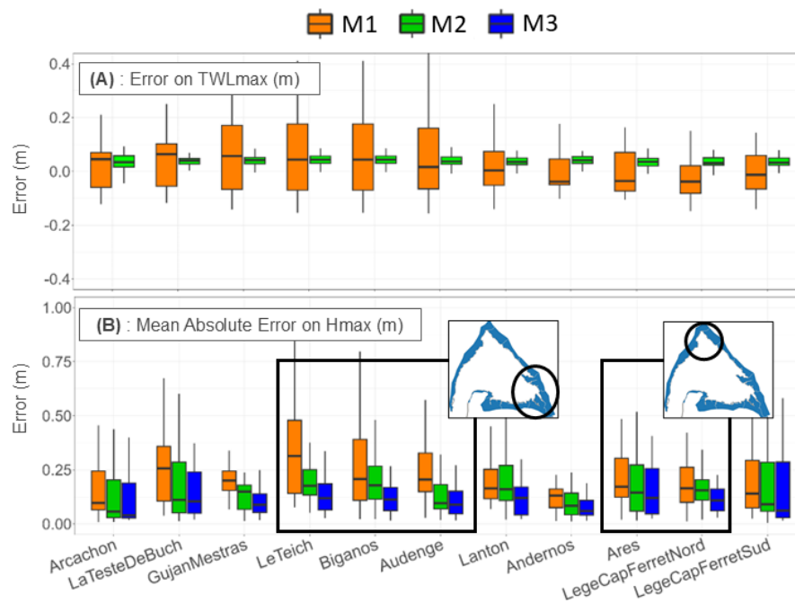
Figure 9. Errors on TWL_{max} (A) and Mean Absolute Errors on H_{max} by restricting the analysis to the mesh nodes that are flooded, i.e. for H_{max} > 0 , in the numerical simulation (B) calculated with the validation cases (Sect. 3.2). Box plots represent the 25th and 75th percentiles.
