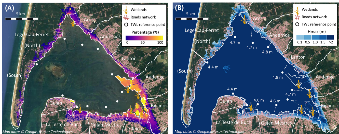
Figure 5. (A) Percentage of scenarios (calculated from the learning database) leading to marine flooding on each node of the model mesh. (B) Water levels denoted TWL_{\max} on the municipalities reference points and Marine flooding map ( H_{\max} ) for the most intense scenario. Map data: © Google, Maxar Technologies.
