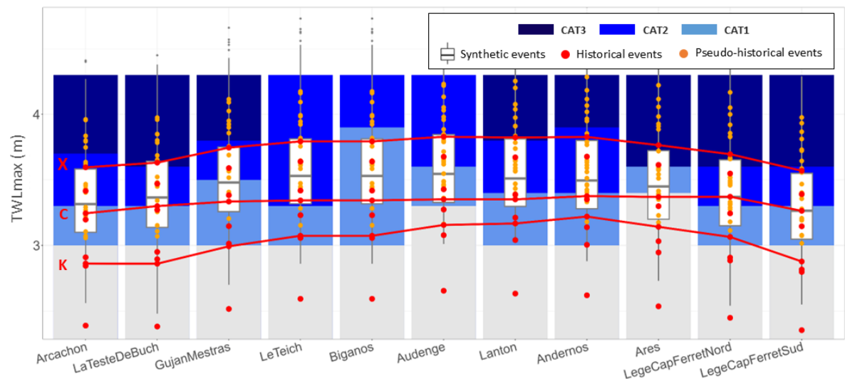
Figure 6. Categories of impact (CAT) related to TWL_{max} and repartition of the scenarios of the datasets: synthetic (box plots), historical (red points) and pseudo-historical (orange points). Red lines illustrate the variations of TWL_{max} for Klaus (K), Céline (C) and Xynthia (X).
