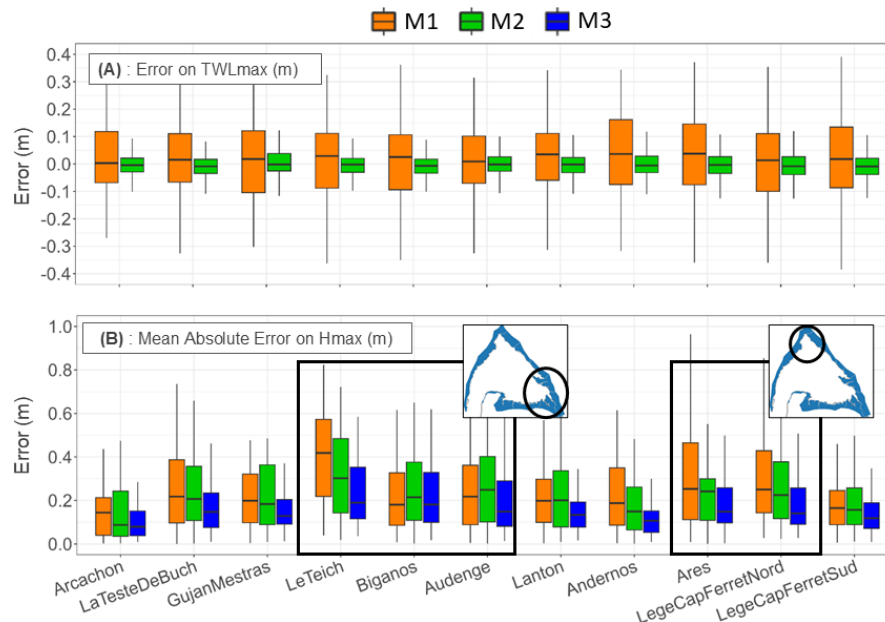
Figure 8. Error on TWL_{max} (A) and Mean Absolute Errors for H_{max} by restricting the analysis to the mesh nodes that are flooded, i.e. for H_{max} > 0 , in the numerical simulation (B) calculated with the 10-fold cross validation (Sect. 3.2). Box plots represent the 25th and 75th percentiles.
