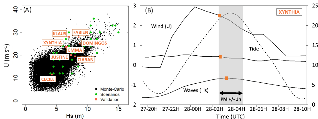
Figure 2. (A) Monte-Carlo simulations (black points), synthetic (green points) and historical or validation (orange points) storm conditions at high tide. (B) Example of storm parameters time series and extraction of conditions at high tide (orange points) for storm Xynthia (2010).
