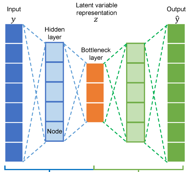
Figure B1. Typical autoencoder architecture.
