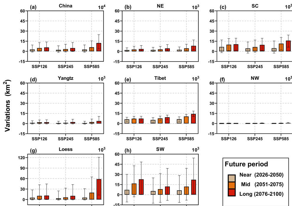
Figure 9. Changes in the area of regions with median to very high landslide susceptibility within inhabited areas of China under different future periods and SSPs, relative to the baseline period. Bars represent the multimodel ensemble mean changes, and error bars indicate the 95 % confidence interval of the ensemble mean.
