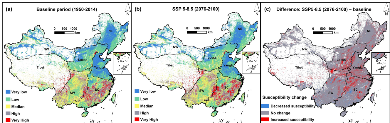
Figure 8. Spatial pattern of landslide susceptibility within inhabited areas of China during (a) the baseline period (1950–2014), and (b) the long-term future (2076–2100) under the SSP5-8.5, and (c) the spatial change in susceptibility between the two periods. In panel (c), increased susceptibility indicates that the susceptibility class under SSP5-8.5 is higher than that during the baseline period, no change indicates that the susceptibility class remains unchanged, and decreased susceptibility indicates that the susceptibility class becomes lower.
