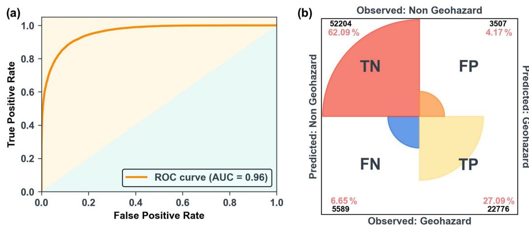
Figure 4. Performance evaluation of the RF model. (a) The ROC curve demonstrates the model’s classification capability, with an AUC of 0.96. (b) The confusion matrix provides a detailed breakdown of the prediction results, including the numbers of correctly and incorrectly classified samples in each category.
