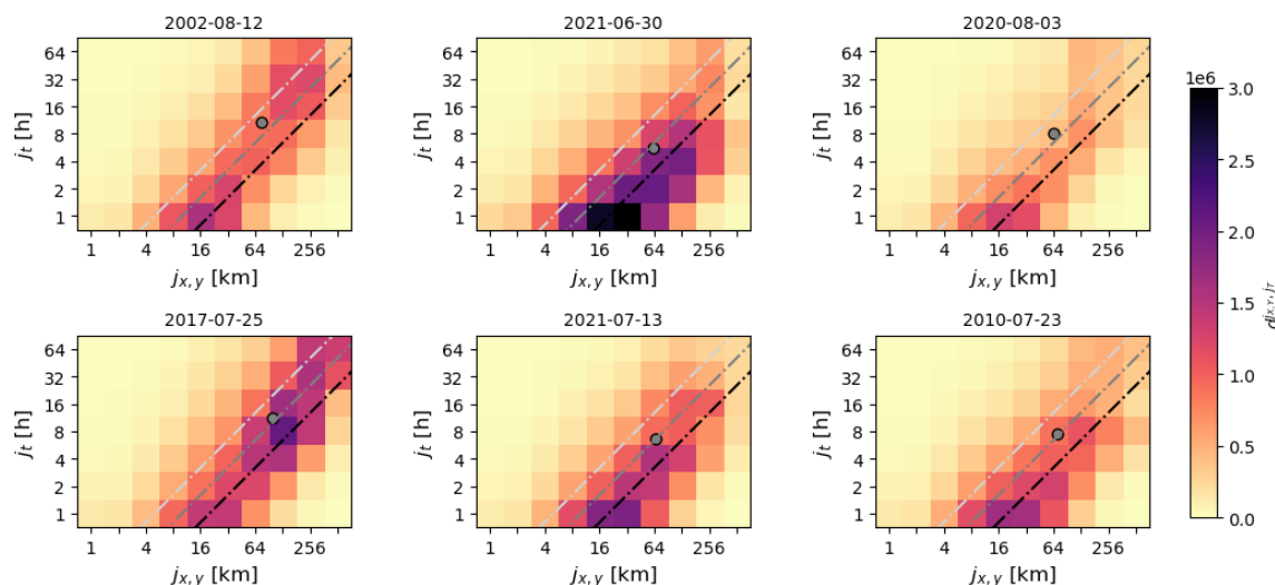
Figure 4. Wavelet spectrum (Eq. 9) of the top six precipitation events identified Sect. 3. The lightgray, gray and black solid lines denote a characteristic speed of 5, 10 and 20 \text{km h}^{-1} . The centre of mass (Eq. 10) is indicated by a gray dot.
