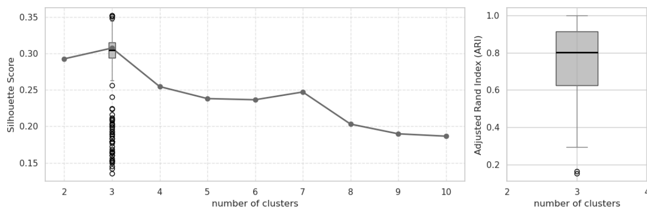
Figure A1. Silhouette score (left) and Adjusted Rand Index (ARI, right) for K -means clustering of the wavelet spectra of the top 100 precipitation events identified in Sect. 3. The silhouette score is shown for cluster sizes ranging from k = 2, \dots, k = 10 . The boxplots are based on a fixed number of three clusters and represent the distribution of silhouette scores and ARI values calculated from 1000 random subsamples (each comprising 80 % of original data).
