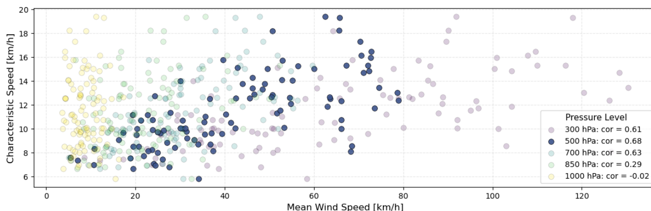
Figure 7. Scatter plot of the characteristic speed derived from the WT vs. the mean wind speed from ERA5 reanalysis at pressure levels of 300, 500, 700, 850, and 1000 hPa. Shown are the top 100 precipitation events identified in Sect. 3. Pearson correlations between characteristic and mean wind speeds are shown in the colorbar labels.
