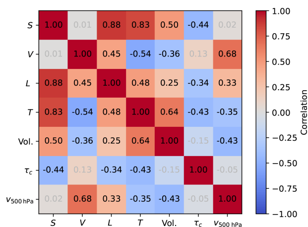
Figure 8. Pearson correlations between WT-derived characteristics ( S , V , L , T ), precipitation volume, convective timescale \tau_c and mean wind speed in 500 hPa. Grey numbers indicate non-significant correlations at p = 0.05 assessed with a permutation test (1000 permutations).
