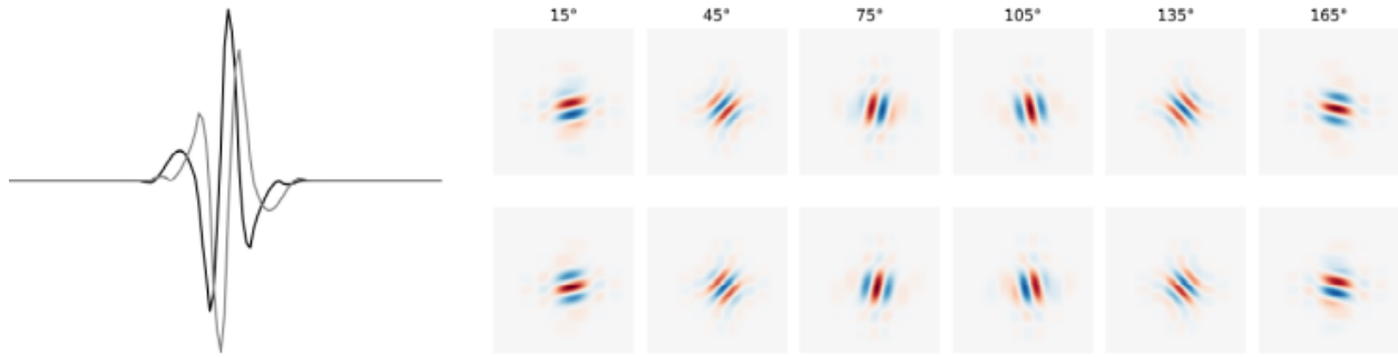
Figure 1. Illustration of the complex Dual-Tree wavelet in one (left) and two dimensions (right). In one dimension, the real and imaginary parts of the wavelet are shown by the black and gray lines, respectively. In two dimensions, the real and imaginary components are displayed in the top and bottom rows, with columns corresponding to different wavelet orientations (15, 45, 75, 105, 135 and 165°).
