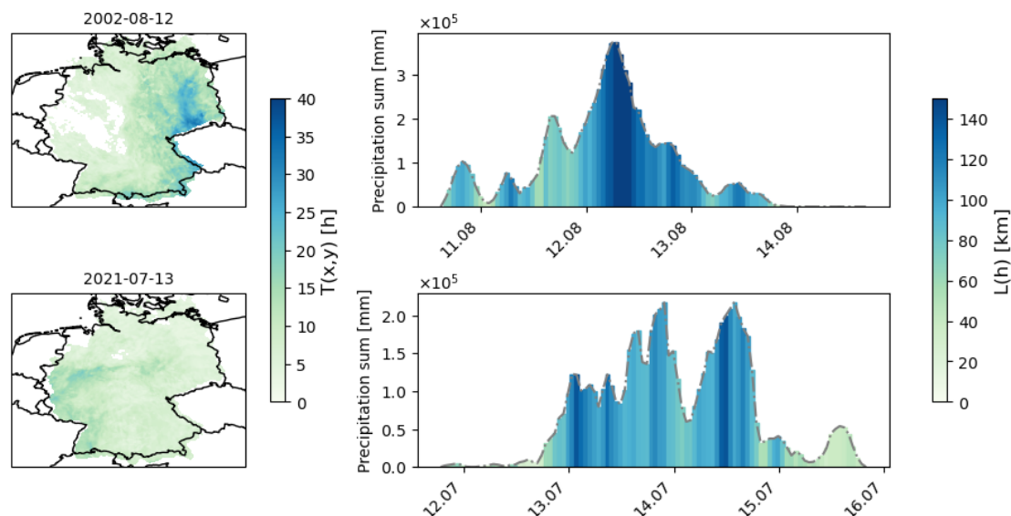
Figure 3. Characteristic time T(x, y) (left) and precipitation sum with colour indicating the characteristic length L(t) (right). Shown are the two precipitation events August 2002 (upper row; based on data from 10 August 2002 16:00 UTC to 14 August 2002 17:00 UTC) and July 2021 (lower row; based on data from 11 July 2021 20:00 UTC to 15 July 2021 21:00 UTC). The precipitation sum is calculated as the total sum of precipitation amount over the respective time period and across Germany.
