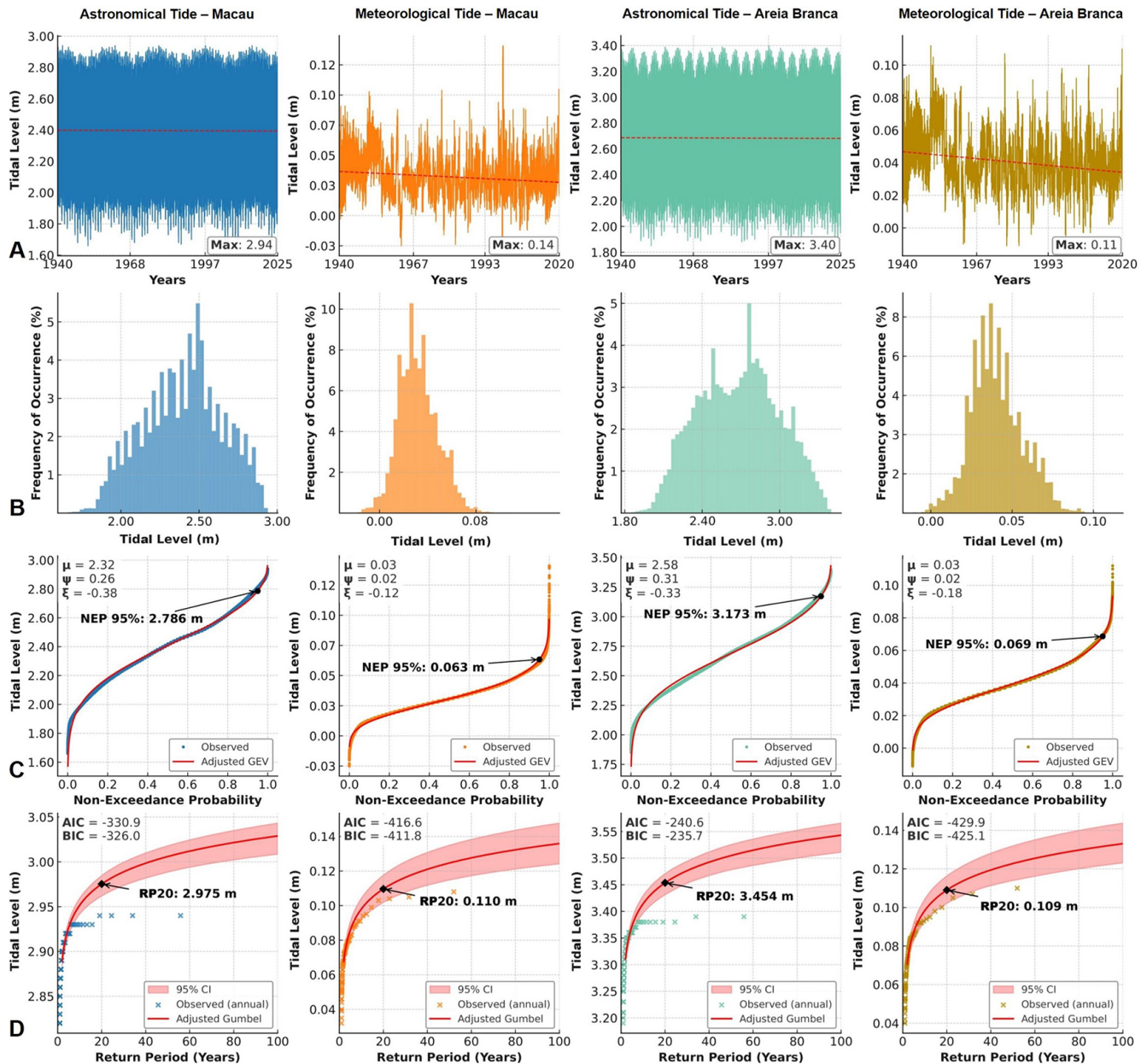
Figure 5. Time series (A), frequency distributions (B), non-exceedance probability curves (C), and return period estimates (D) of maximum astronomical and meteorological tides at Macau and Areia Branca. Each column in the graphs represents a location and the type of tide analysed.
