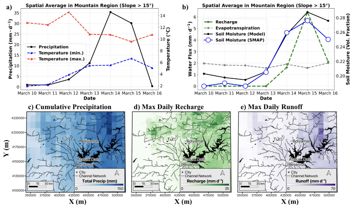
Figure 4. Landlab land surface model response to the 14–15 March AR event: (a) Spatial averages of meteorological forcing of 10–16 March including IMERG precipitation and ERA5 temperature time series. (b) Modeled local recharge, soil moisture, and evapotranspiration as well as SMAP L4 soil moisture observations. (c) Cumulative IMERG precipitation of the 7 d period, (d, e) modeled spatial maximum daily upslope average recharge ( R ) and local runoff ( Q ). Time series are spatial averages of the domain filtered for slopes > 15^\circ to report conditions in the mountainous regions. Max daily R and Q fields are Landlab outputs that are produced from combining the maximum values from the 7 daily response maps to create a composite map of the wettest conditions. All data are projected in WGS 84/UTM Zone 10N (EPSG:32610) for Landlab modeling. IMERG precipitation data © NASA. ERA-5 temperature data © ECMWF/Copernicus. SMAP-L4 soil moisture data © NASA.
