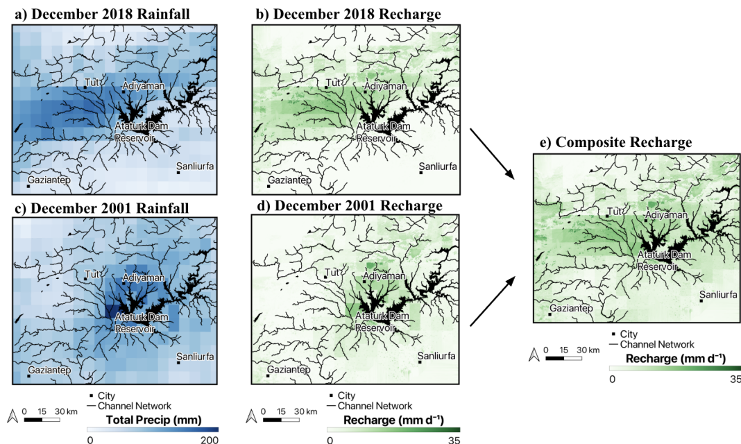
Figure 9. Cumulative rainfall and composited local maximum upslope average recharge for: (a, b) December 2018 and (c, d) December 2001 rainfall events; and (e) the composite recharge rate field of the combined pre-March 2023 extreme events identified in the IMERG catalog. Max daily recharge rate fields are derived from reduction processes outlined in Sect. 3.2 and are representative of the maximum daily recharge observed over the 7 d period for each cell. IMERG precipitation data © NASA.
