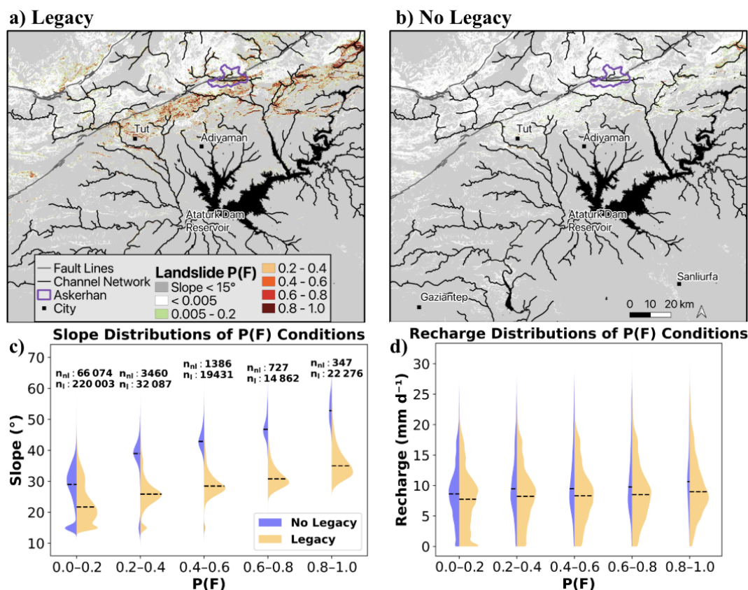
Figure 6. Landslide probability of failure P(F) maps for the central earthquake-impacted area overlain with mapped channel network for slopes greater than 15^\circ : (a) with PGA-dependent legacy effect (Eq. 2) and (b) without legacy effects. (c, d) Comparison of (a) and (b) using violin plots of local slopes and daily R , respectively, for different bins of landslide probabilities, excluding areas of P(F) = 0 . For each probability bin, the number of grid cells classified as legacy ( n_l ) and non-legacy ( n_{nl} ) is indicated in the figure, horizontal dashed lines indicate the median value.
