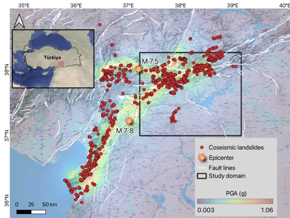
Figure 1. USGS ShakeMap raster composition which consists of PGA resulting from the two major earthquakes of magnitude M_w 7.8 and M_w 7.5 (exclusive of aftershocks) occurring along the East Anatolian fault zone. The coseismic landslide inventory, marked by red circles, is provided by Görüm et al. (2023), while the active faults, indicated by white lines, are mapped by Emre et al. (2013). ShakeMap PGA data © USGS. Active fault data © MTA (General Directorate of Mineral Research and Exploration, Türkiye).
