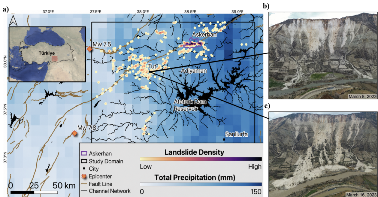
Figure 2. (a) NASA's Integrated Multi-satellite Retrievals for GPM (IMERG) precipitation estimates for 10–16 March 2023. This atmospheric river swept through the central earthquake impacted area, delivering up to 146.4 mm of rainfall over a 7 d span. Photos captured within the town of Tut illustrate the landscape effects of (b) coseismic driven crown cracking and landsliding and (c) post-seismic storm-driven sedimentation and debris flow (Görüm et al., 2025). A 10 km 2 validation site within the Askerhan subcatchment, where a high density of post-seismic landslides were observed, was selected for model validation. IMERG precipitation data © NASA.
