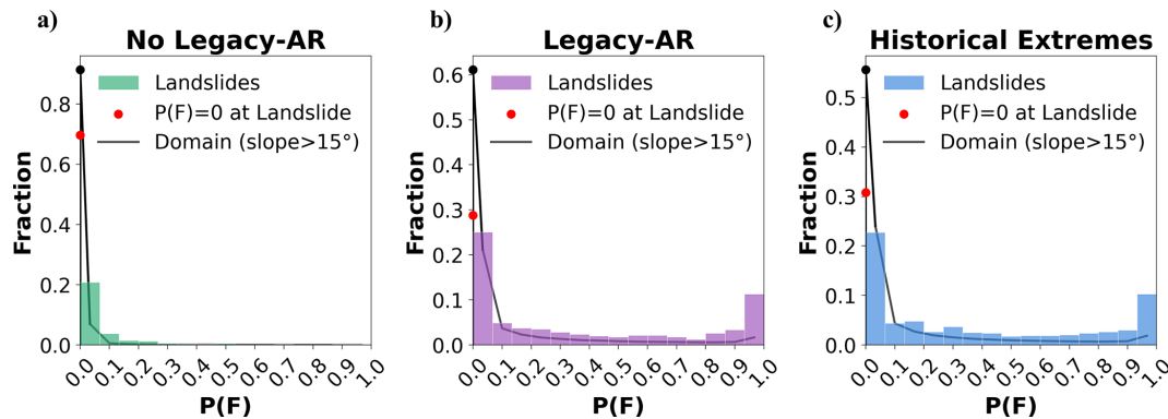
Figure 11. Distribution of modeled probability of failure, P(F) , across the model domain for three post-seismic 14–15 March AR event scenarios (black lines), and distribution of P(F) at mapped landslide locations (colored bars): (a) without earthquake legacy; (b) with earthquake legacy; (c) earthquake legacy combined with historical extremes as forecast model. Large points at P(F) = 0 indicate the fraction of the domain and mapped landslide locations predicted stable. The figure illustrates the shift from near-zero probabilities in the no-legacy case toward more realistic, moderate-to-high probabilities when earthquake legacy effects are included, and the similar probability structure reproduced by the historical-extremes model. Landslide data used is composed of 90 % coseismic and 10 % post-seismic landslides.
