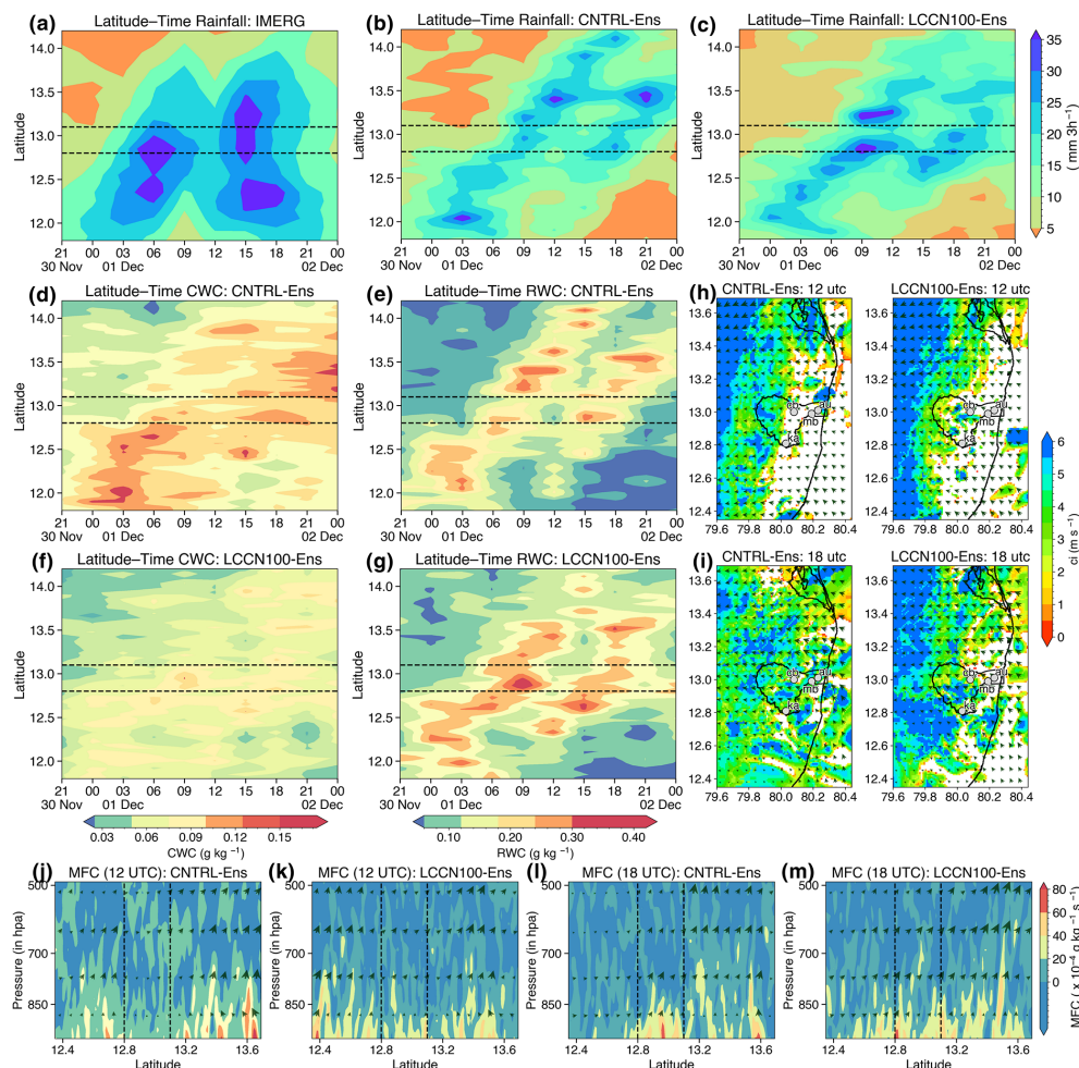
Figure 3. Aerosol-Induced Convection in the Region (dotted lines indicate basin extent). The top row indicates latitude-temporal precipitation for (a) IMERG (b) CNTRL-Ens and (c) LCCN100-Ens from 30 November 21:00 UTC–2 December 00:00 UTC. The two middle rows (left and middle columns) show altitude-averaged latitude-time variations of (d, f) cloud water (CWC) and (e, g) rainwater content (RWC) for CNTRL-Ens (d–e) and LCCN100-Ens (f–g) during the same period. The right column displays the spatial distribution of cold pool intensity for CNTRL-Ens and LCCN100-Ens at (h) 12:00 and (i) 18:00 UTC. In the bottom row, panels present longitude-averaged latitude-altitude profiles of moisture flux convergence and winds at the 12:00 UTC (j–k) and 18:00 UTC (l–m) on 1 December for CNTRL-Ens (j, l) and LCCN100-Ens (k, m).
