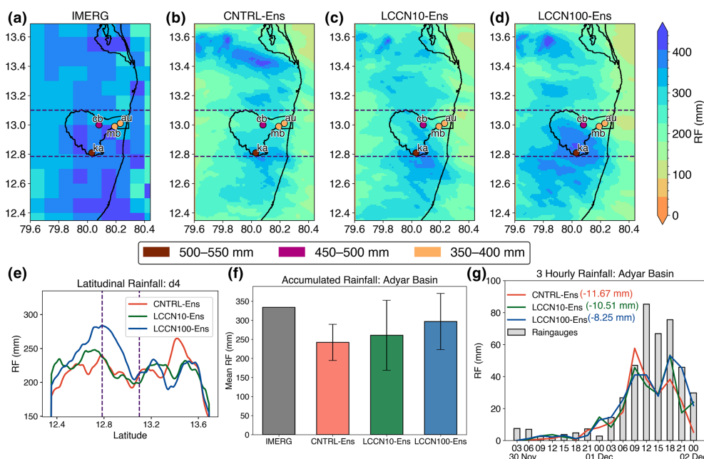
Figure 2. Spatio-temporal distribution of rainfall across sensitivity experiments (dotted lines indicate basin extent). Panels show: (a) IMERG-derived accumulated rainfall, (b)–(d) Accumulated rainfall from CNTRL-Ens, LCCN10-Ens, and LCCN100-Ens, respectively, with rain gauge locations and observed totals at Kattupakkam (ka), Chembarambakkam (cb), Meenambakkam (mb), and Anna University (au) within the basin. (e) Latitudinal distribution of accumulated rainfall. (f) Basin-averaged accumulated rainfall from IMERG and sensitivity experiments (error bars showcasing variation in ensemble members) (g) 3-hourly temporal rainfall patterns with mean biases at Adyar basin. An average of four rain gauges have been used for temporal comparison.
