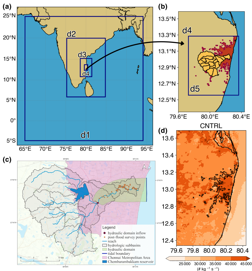
Figure 1. WRF simulation domains, emission distribution, and HEC-HMS, HEC-RAS domain for Flood Analysis. (a) The nested parent domains used in WRF simulations. (b) The inner domains (d4 and d5) with urban land use and Adyar basin. (c) The delineated basin and stream network in HEC-HMS, as well as the hydraulic domain and boundary conditions for HEC-RAS. It also shows the locations where the post-flood survey was conducted to obtain the maximum inundation depths for the 2015 floods. (d) CCN surface emissions with urban land use for CNTRL in d4.
