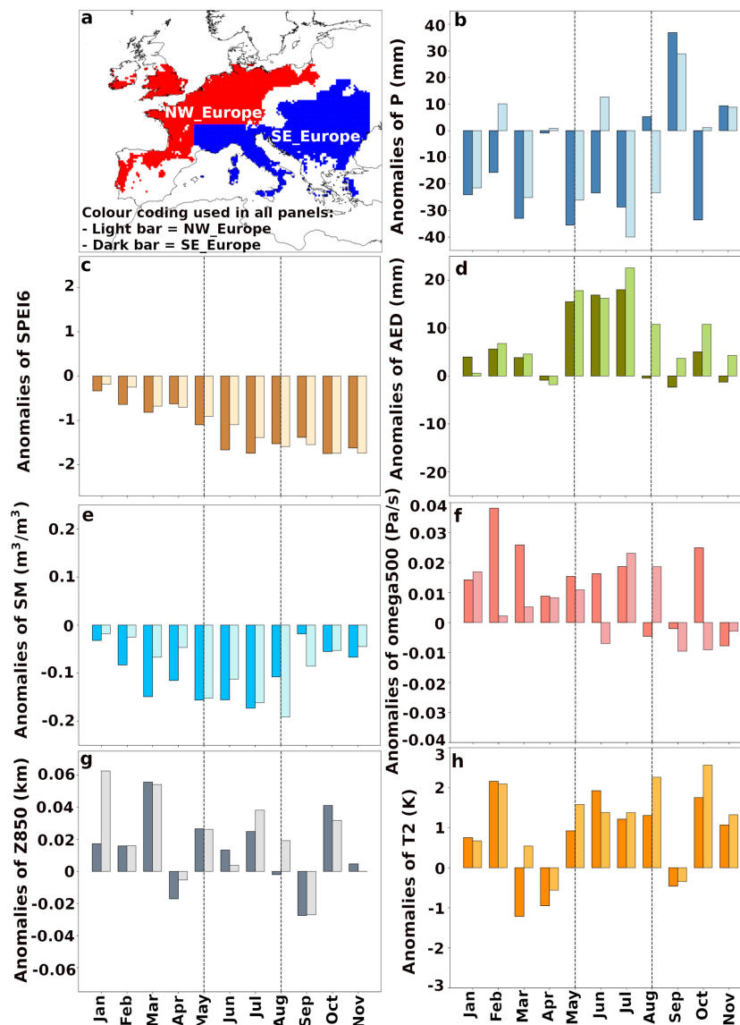
Figure 1. Target regions and hydro-climatic monthly anomalies during the 2022 European drought. (a) Target regions considered in this study: northern-western Europe (NW_Europe, red) and southern-eastern Europe (SE_Europe, blue). (b–h) Monthly averaged anomalies of key hydro-climatic variables, calculated relative to the 1994–2023 climatology using ERA5 reanalysis data: (b) accumulated precipitation (P, mm); (c) 6-month Standardized Precipitation–Evapotranspiration Index (SPEI6); (d) atmospheric evaporative demand (AED, mm); (e) soil moisture (SM, \text{m}^3 \text{m}^{-3} ); (f) vertical velocity at 500 hPa (omega500, \text{Pa s}^{-1} ); (g) geopotential height at 850 hPa (Z850, km); and (h) 2 m temperature (T2, K). Colour intensity indicates each region: higher intensity for SE_Europe and lower intensity for NW_Europe. The framed period highlights the active hydro-climatic drought peak period (May–August 2022). The spatial patterns and corresponding anomalies used to determine the monthly anomaly series are shown in Figs. S1–S3.
