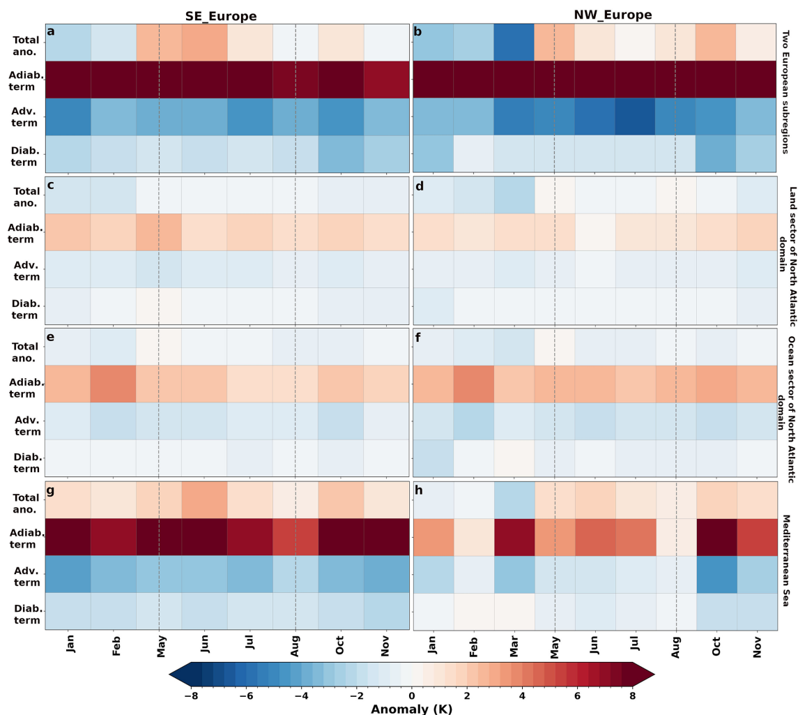
Figure 3. Monthly series of temperature anomaly sources during the 2022 European drought. Heat maps show monthly anomalies of total temperature, and of the adiabatic, diabatic and advective components from January to November 2022. Left and right panels display anomalies for the SE_Europe and NW_Europe subregions, respectively. Panels show the anomaly values averaged over (a, b) each of the two European subregions, (c, d) the North Atlantic land sector, (e, f) the North Atlantic oceanic sector, and (g, h) the Mediterranean Sea. The framed period highlights the active hydro-climatic drought peak period (May–August 2022). Anomalies are computed relative to the 1994–2023 climatology. Data processed from FLEXPART outputs forced by ERA5 data.
