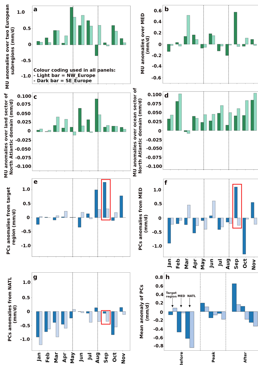
Figure 2. Moisture uptake (MU) and precipitation contributions (PCs) associated with the 2022 European drought. Colour bar intensity indicates each European subregion: higher intensity for SE_Europe and lower intensity for NW_Europe. The framed period highlights the peak drought months (May–August 2022). (a–d) MU monthly anomalies (in \text{mm d}^{-1} , green plots) computed over: (a) each European subregion; (b) the Mediterranean Sea; (c) land; and (d) ocean sectors of the North Atlantic domain. (e–h) Monthly anomalies of PCs (mm/day, blue bars) from: (f) the Mediterranean (MED) moisture source; (g) the NATL; and (e) the two European subregions. The red rectangle indicates the month considered the drought-breaking month, September 2023. (h) Average PCs anomaly for each source for the periods Before (January–April), Peak (May–August), and After (September–November). The framed period highlights the active hydro-climatic drought peak period (May–August 2022). The period considered for the calculation of the anomalies is 1994–2023, and the spatial patterns and corresponding anomalies used to determine the monthly anomaly series are shown in Figs. S6–S8.
