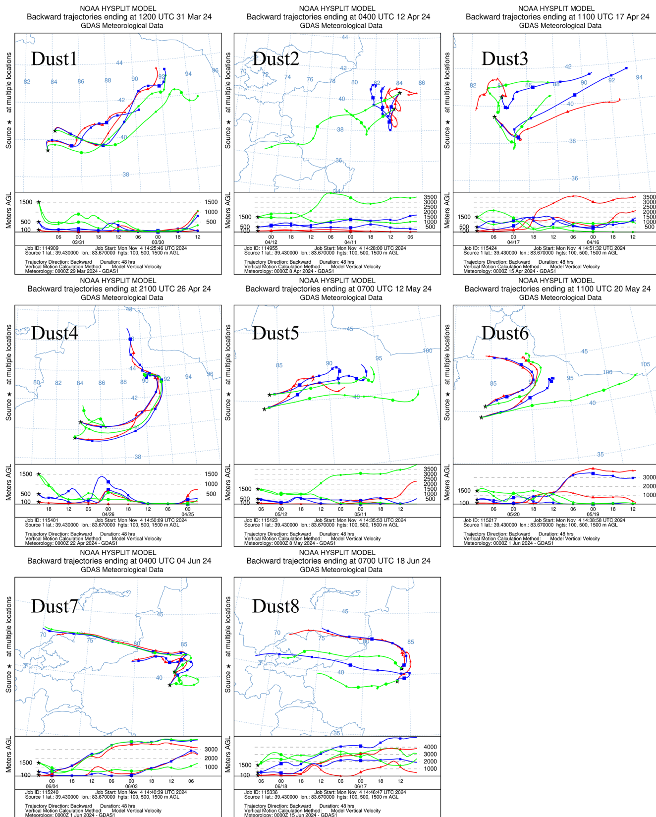
Figure 2. Backward trajectories of the eight dust-storm events.
