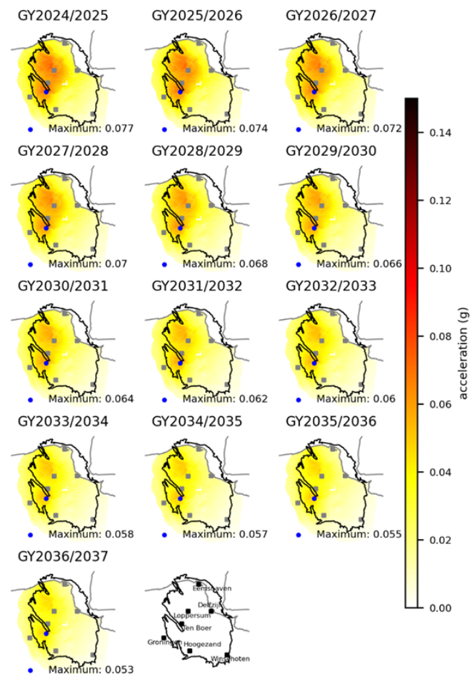
Figure 15. Peak Ground Acceleration (pseudo-spectral acceleration at 0.01 s) hazard map for a 475 return period (10 % probability of exceedance in 50 years). The blue dot indicates the position of the largest hazard for each year. Base case (no injection).
