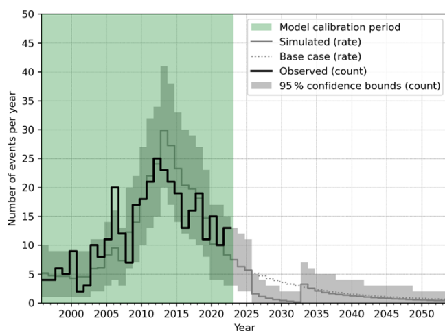
Figure 13. As Fig. 7, except for the LO-10ZB-7Y scenario.
