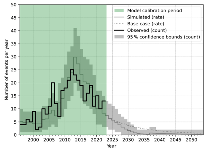
Figure 14. As Fig. 7, except for the SE-10ZB-11Y scenario.
