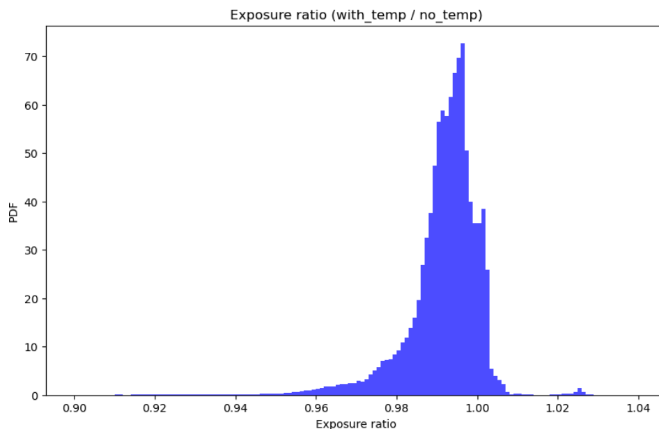
Figure A10. Ratio between risk level (Local Personal Risk) computed with temperature effects and without temperature effects. For each building, for each year in the forecast, and for each scenario we obtain a ratio. We show this as a single histogram, combining all the annual data of all scenarios in a single plot. In general, the risk level computed per building with temperature effects is a few percent lower than without temperature effects due to the slightly lower levels of seismicity. However, for some select buildings the ratio is slightly above unity. The main take-away is that the effect of accounting for temperature effects is very minor.
