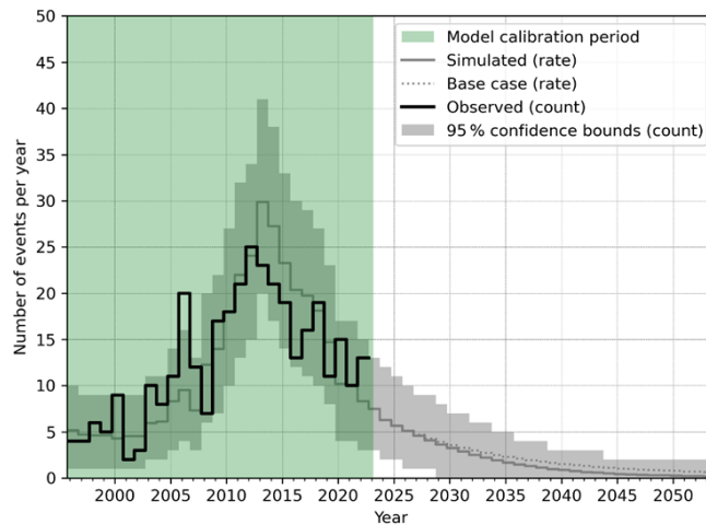
Figure 10. As Fig. 7, except for the SE scenario.
