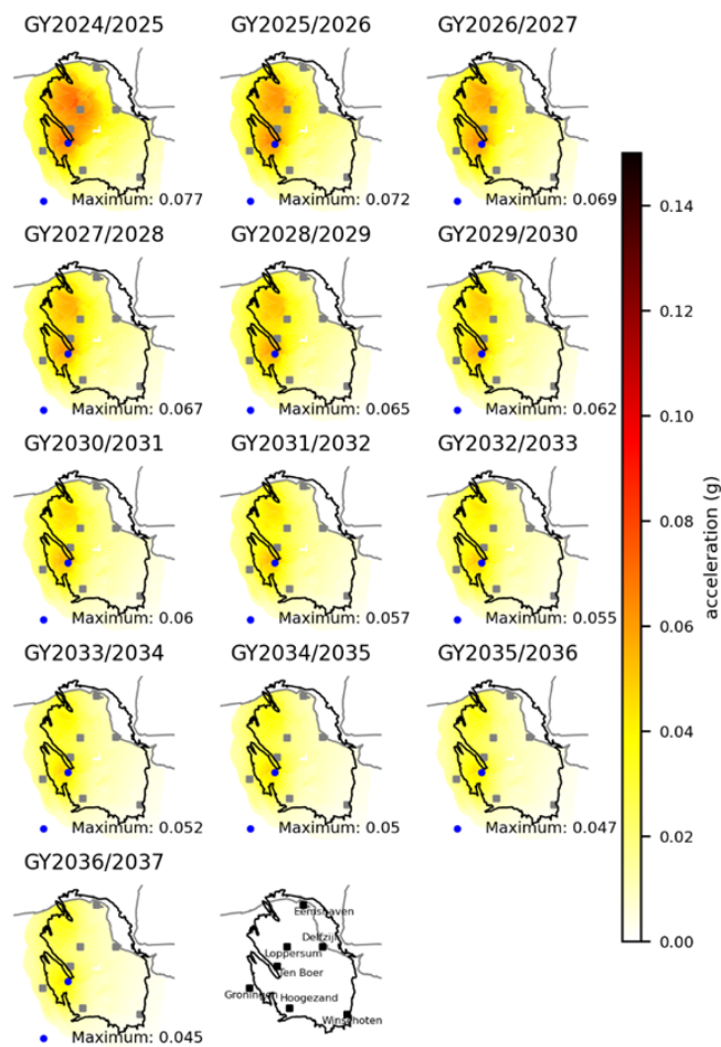
Figure 16. As Fig. 15, but for the LO scenario.
