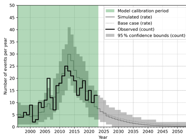
Figure 9. As Fig. 7, except for the LO_SE scenario.
