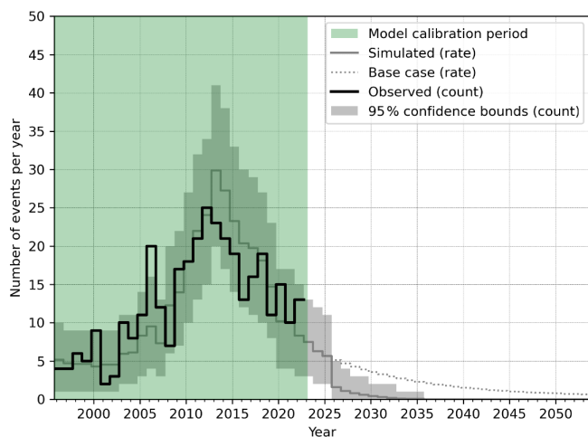
Figure 7. Number of events per year in the Groningen field of magnitude M 1.5 and above for the LO-10ZB scenario (with temperature effects included). The solid grey line is the modelled expected number of events, the grey area gives the 95 % confidence bounds per year. The solid black line is the historically observed event rate and the green area is the period over which the model is calibrated. The dotted reference line represents the base case for comparison.
