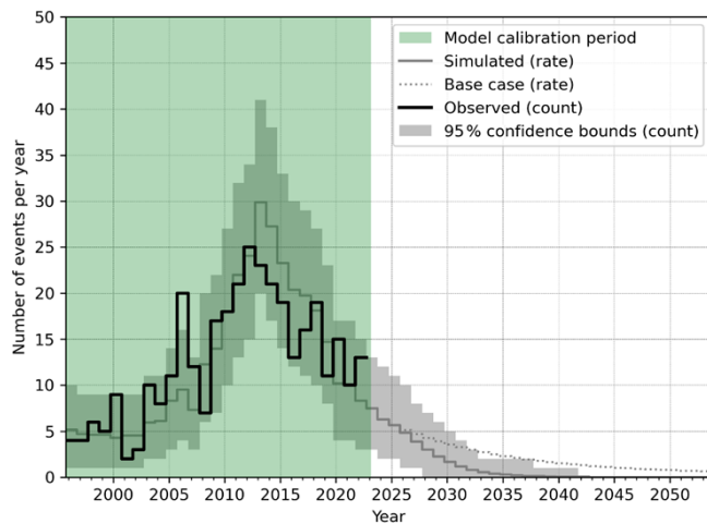
Figure 12. As Fig. 7, except for the SE-10ZB scenario.
