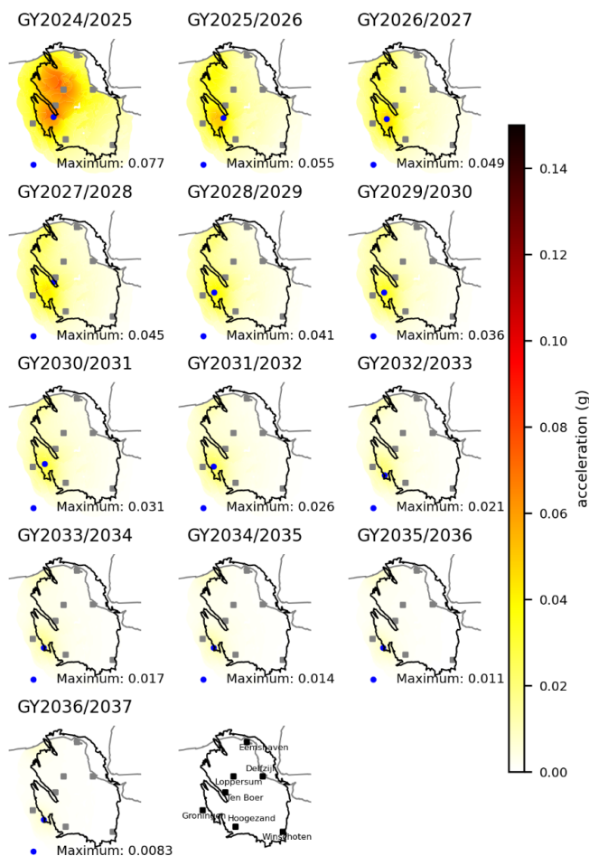
Figure 17. As Fig. 15, but for the LO-10ZB scenario.
