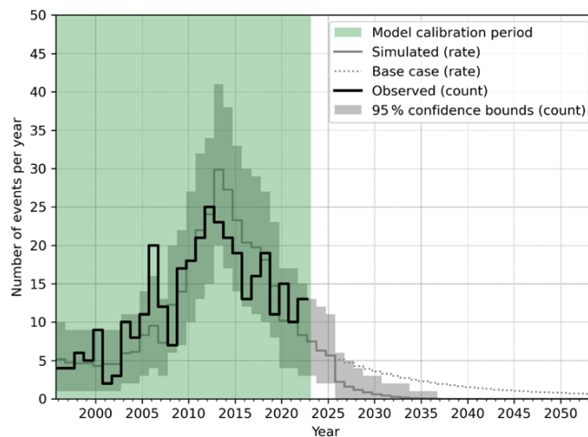
Figure 11. As Fig. 7, except for the LO_SE-10ZB scenario.
