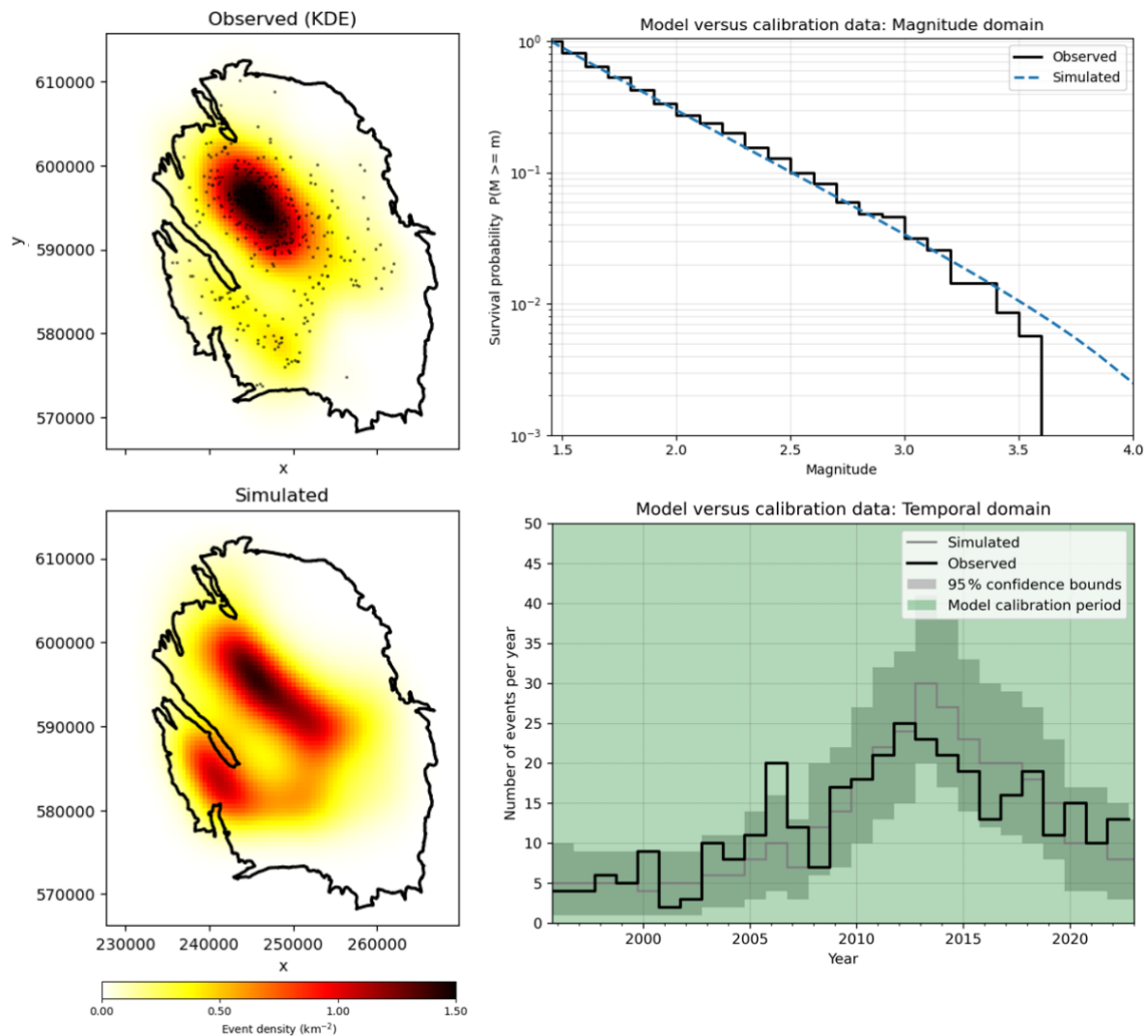
Figure 6. A comparison between the calibrated model and the calibration data. On the left side of the figure: the observed spatial distribution of events (top) vs. the modelled spatial distribution. On the top right side of the figure: the observed magnitude distribution vs. the modelled magnitude distribution. On the bottom right side of the figure: the observed temporal distribution vs. the modelled temporal distribution.
