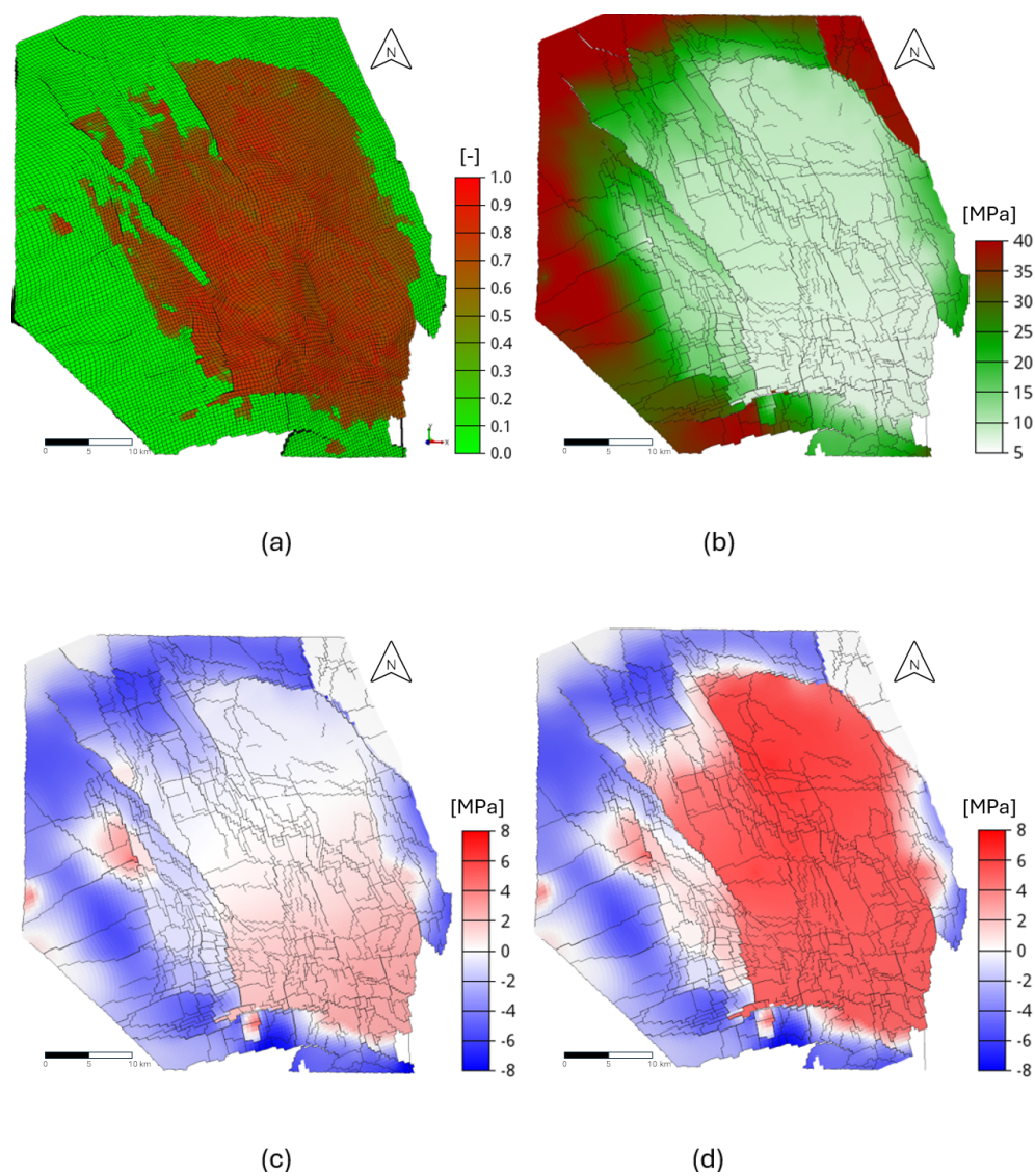
Figure 3. (a) Top view of the initial gas saturation [–] on the simulation grid. (b) Pressure [MPa] at the end of production (October 2023). (c) Change in pressure [MPa] over the injection period for the SE scenario. (d) Change in pressure [MPa] over the injection period for the LO_SE-10ZB scenario.
