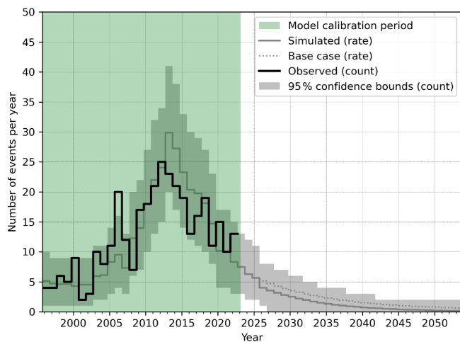
Figure 8. As Fig. 7, except for the LO scenario.
