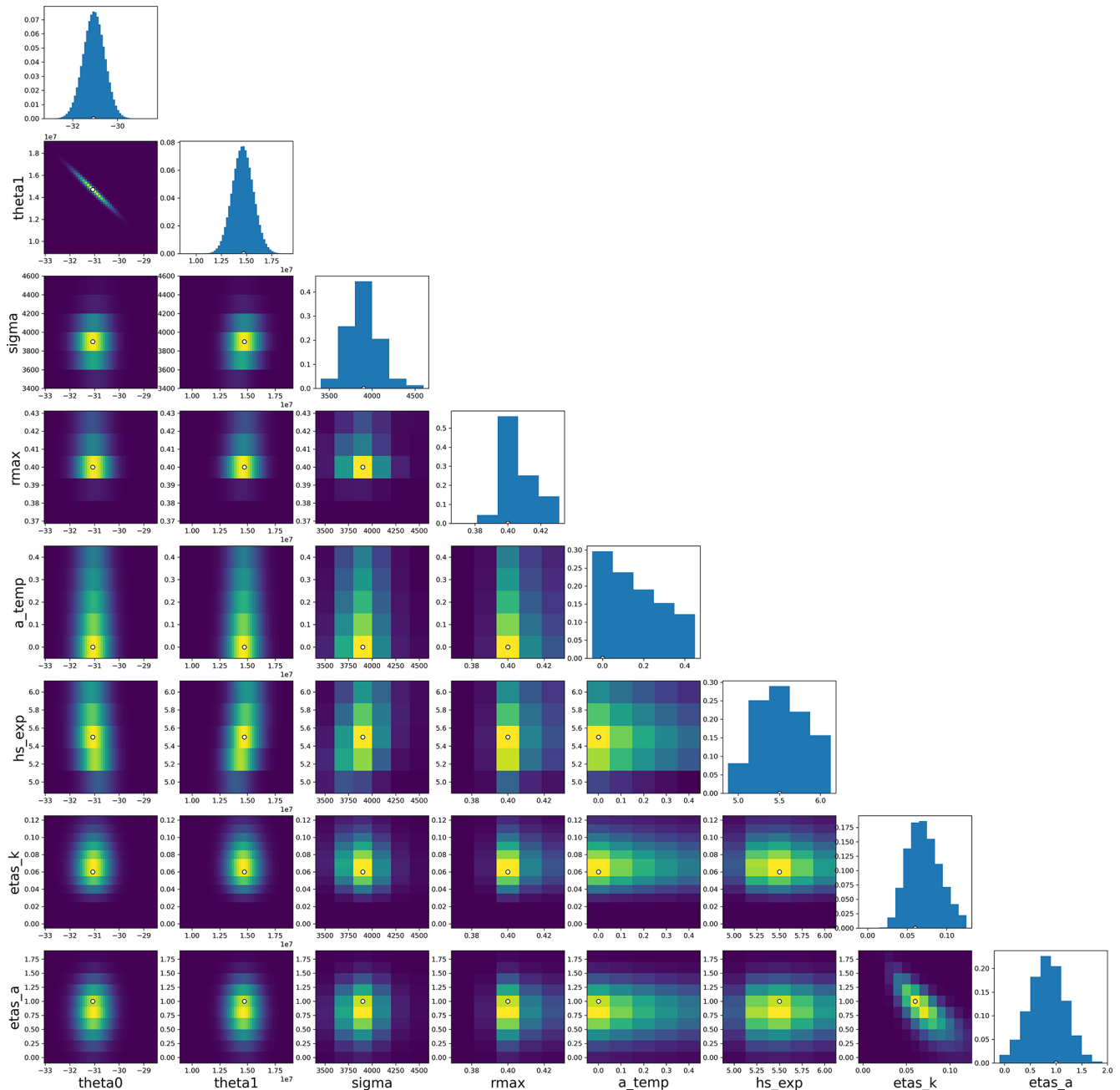
Figure A1. Posterior distribution of the model parameters for the earthquake rate model. See TNO 2020 for a complete overview. We calibrate the model on all observed earthquakes in the Groningen field with M_{\min} = 1.45 over the period 1 January 1995–28 February 2023. The new parameter which relates to the impact of temperature changes on seismicity ( a_T or a\_temp in this figure) has been assigned a uniform prior probability over the range zero (no effect of temperature) to 0.4 \text{ MPa K}^{-1} (which corresponds to high sensitivity to temperature changes, \alpha_T = 2.4 \times 10^{-5} \text{ K}^{-1} for E = 15 \text{ GPa} and \nu = 0.2 ). The posterior distribution for a_T clearly shows a peak in probability density/mass at a_T = 0 and a rapidly decreasing probability density for higher values of a_T . This indicates that even based on the limited past temperature changes, the model performs better when these temperature changes do not result in seismicity.
