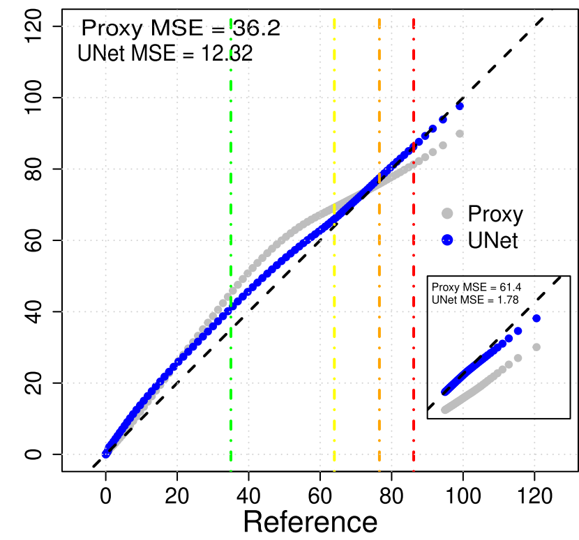
COASM QQ Plot: Proxy vs UNet
