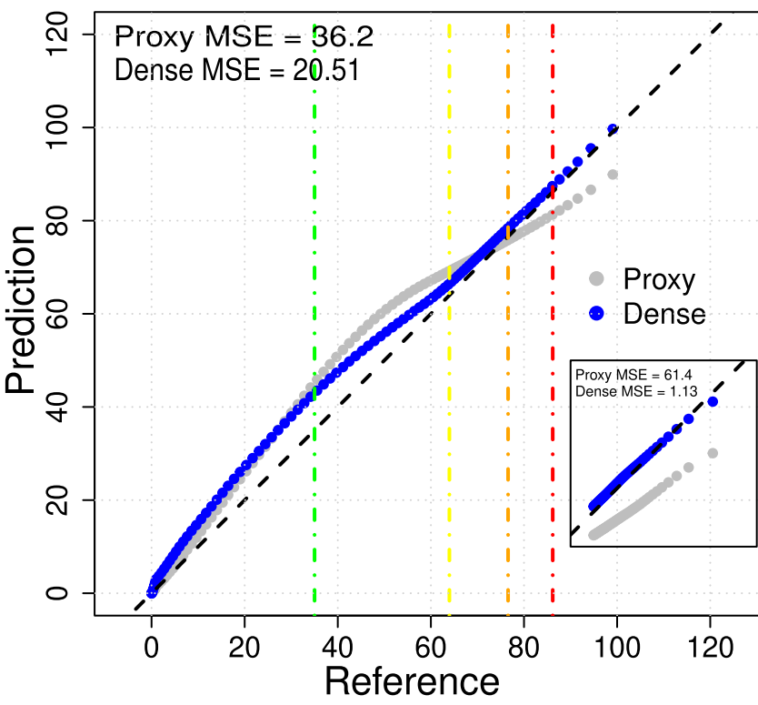
COASM QQ Plot: Proxy vs Dense
