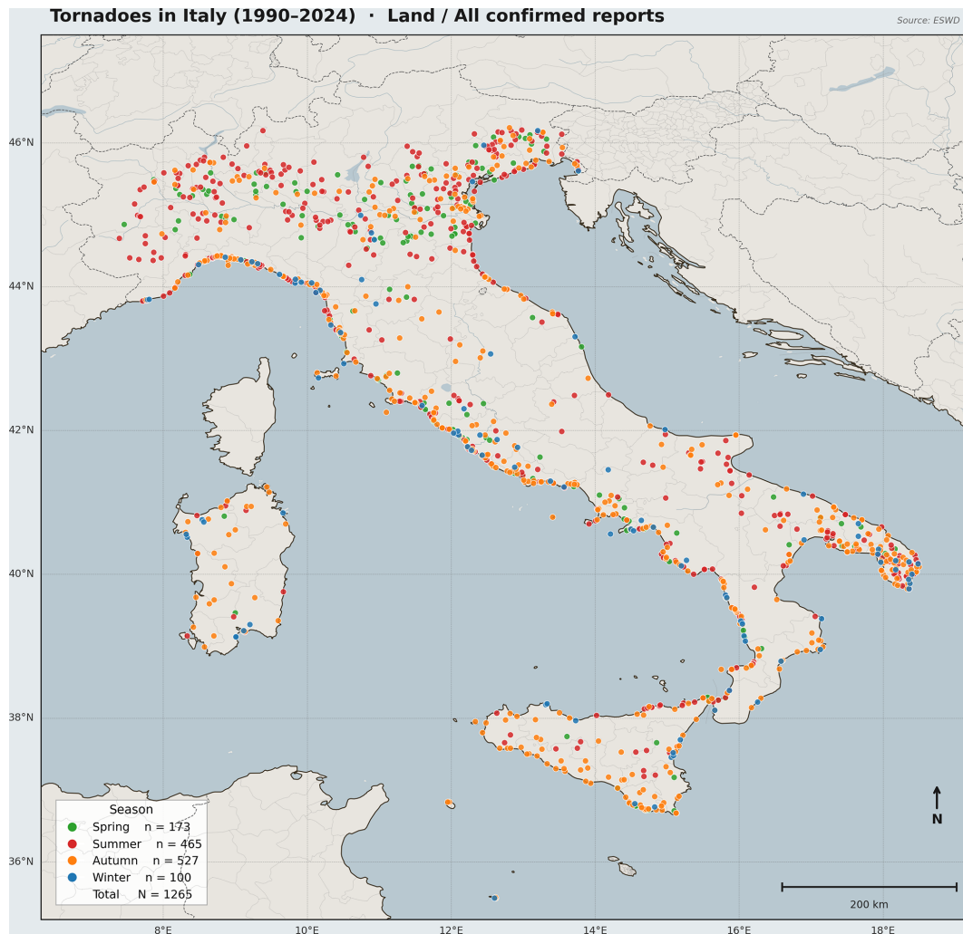
Figure 5. Map of selected Italian tornadoes crossing “land” for the period 1990–2024; different colors represent the seasons (reports derived from © European Severe Storms Laboratory (ESWD). All rights reserved).
