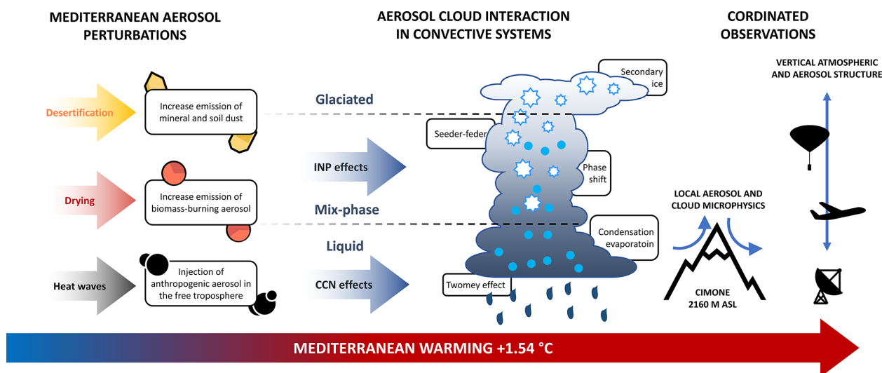
Figure 7. Schematic representing the aerosol cloud interactions (ACI) under the warming scenario in the Mediterranean. The cloud condensation nuclei (CCN) and ice nucleating particles (INPs) trigger different processes during severe storm development. To isolate the ACI contribution, observations of aerosol and cloud microphysics must be coordinated with vertically resolved dynamics observations.
