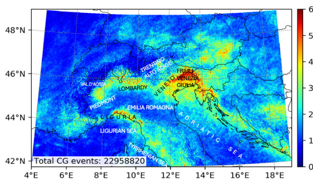
Figure 2. Spatial distribution of Cloud-to-Ground lightning (per km 2 yr) based on EUCLID data from 2005 to 2019 (adapted from Manzato et al., 2022a). The location of northern Italian regions is also shown.
