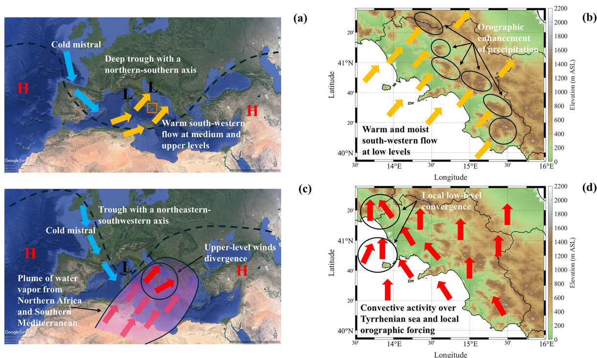
Figure 4. Schematic illustration of two of the six large-scale configurations associated with heavy-precipitation events in the Campania Region (southern Italy) identified by Capozzi et al. (2023a). Panels (a) and (b) show Pattern 1 (warm and moist southwesterly flow and orographic enhancement of precipitation along the main Apennine ranges); panels (c) and (d) represent Pattern 6 (convective activity over the Tyrrhenian Sea and the northern sector under local low-level convergence). In (a) and (c), the black dashed line marks the approximate position of the 552-dam 500 hPa geopotential-height contour, while the orange box in (a) locates the Campania region, zoomed in (b) and in (d). Images credit: © Google Earth, Data Sio, NOAA, U.S. Navy, NGA, GEBCO.
