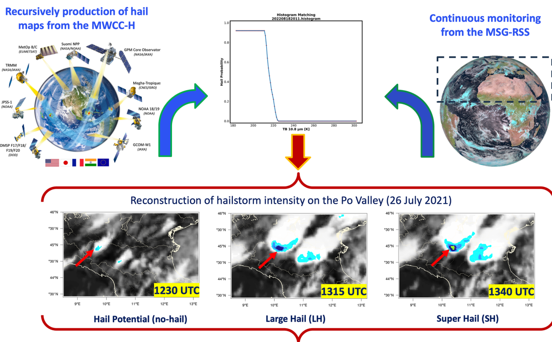
Figure 6. MASHA conceptual scheme (top images; © NASA. All rights reserved. © EUMETSAT. All rights reserved) and highlights of hailstorm evolution affecting Northern Italy on 26 July 2021 (bottom bracketed images).
