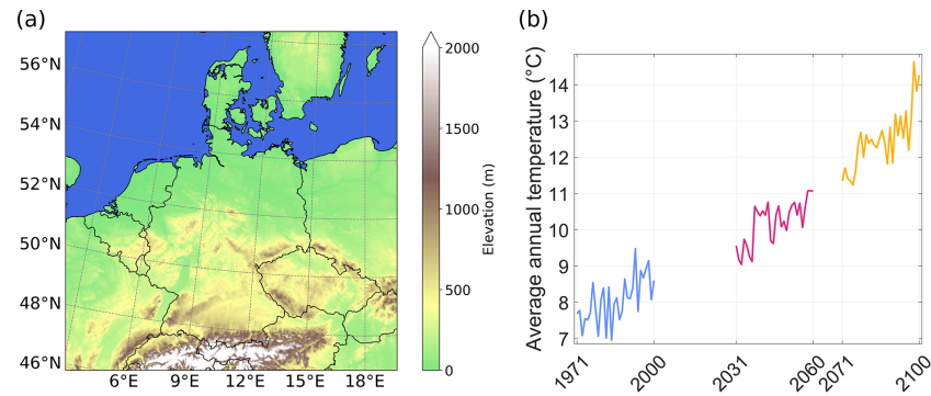
Figure 1. (a) Study area, including 425 \times 415 grid points which are mapped using a rotated pole projection. (b) Time series of the mean annual temperature averaged over the study area considering three 30-year periods.
