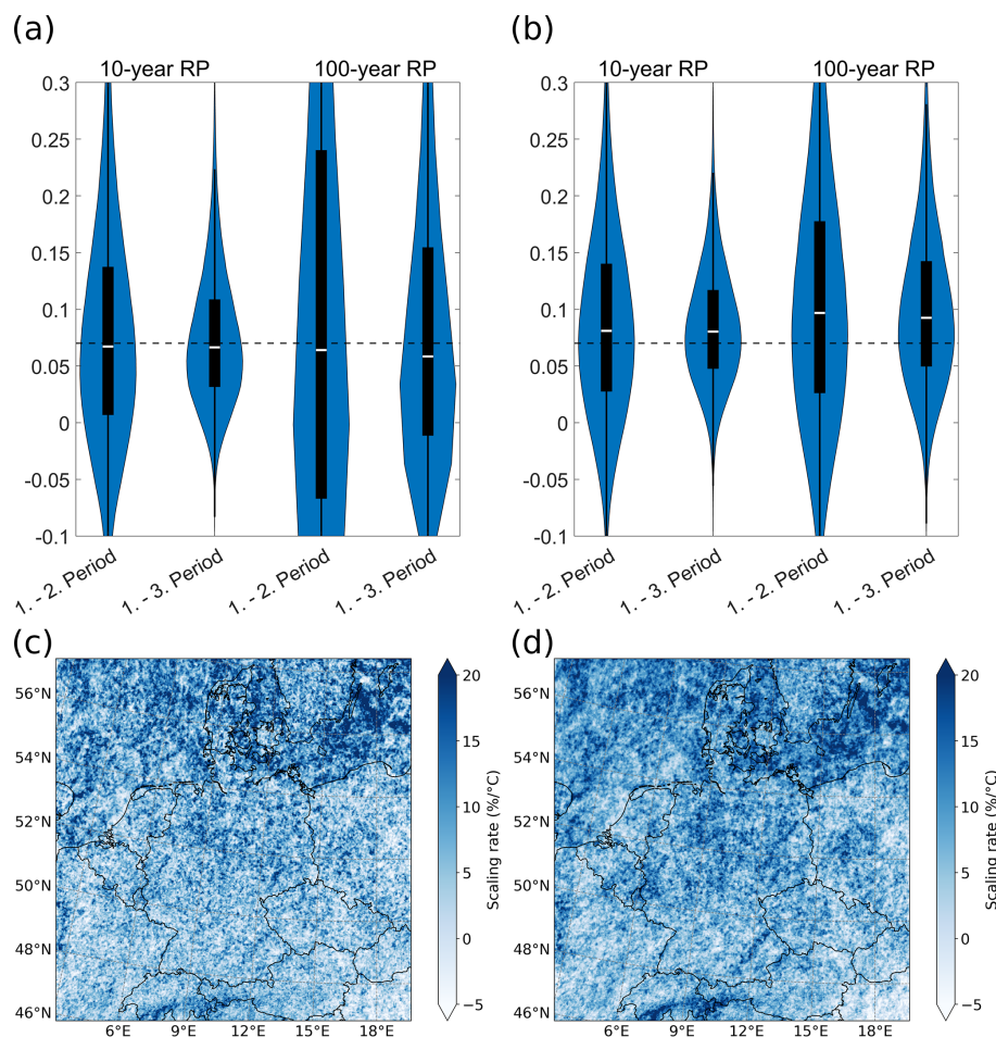
Figure 5. Temperature scaling for the 10-year and 100-year return levels for the GEV (a) and sMEV (b) approach across the study area. For Fig. (a) and (b) the y-axis shows the relative change of the return level per degree of warming, based on the 30-year average temperature of each period. The temperature scaling is shown for the difference between the first and second period as well as the first and third period. Black bars mark the 25th and 75th quantiles with the white marker showing the mean. The dashed line indicates the Clausius-Clapeyron scaling of 7\% \text{ } ^\circ\text{C}^{-1} . Panels (c) and (d) display the 10-year return level change per degree of warming for the GEV (c) and sMEV (d) approach. The rate of change is calculated based on the return levels of the periods 2071–2100 and 1971–2001.
