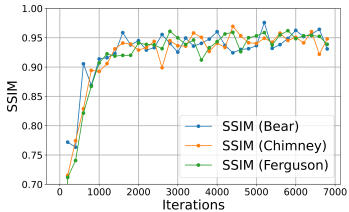
(d) SSIM during validation
