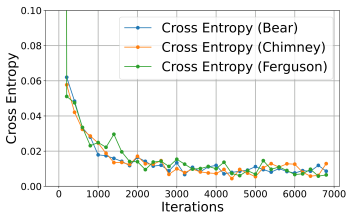
(a) Cross Entropy Loss during training
