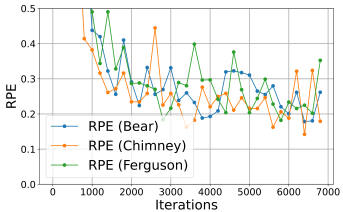
(c) RPE during validation
