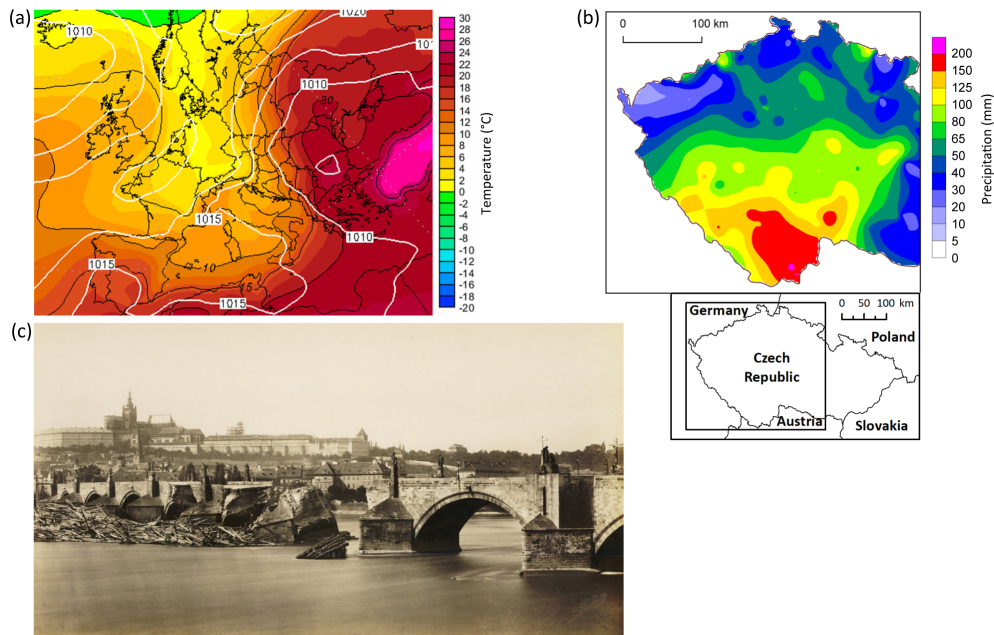
Figure 5. The flood of the Vltava River on 3–4 September 1890 in Bohemia: (a) sea level pressure (hPa) and air temperature at the 850 hPa level on 2 September at 12:00 UTC (Wetterzentrale, 2026); (b) precipitation totals on 1–3 September 1890 in Bohemia; (c) the damaged Charles Bridge on the Vltava River in Prague (source: from the J. Eckert studio, Museum of Prague, catalogue no. H 029.416; cropped).
