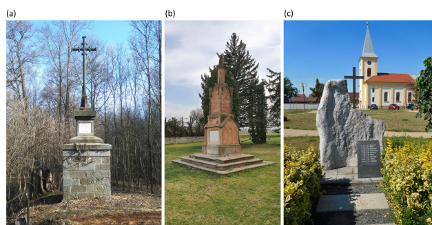
Figure 2. Memorials to fatalities of disastrous events: (a) flood of 25–26 May 1872: the stone cross of seven victims in Stebno (Prudký, 2017); (b) snow of 10 November 1868: the memorial of 22 victims of the train crash in Cerhovice (source: Mapy.com – Mapy, 2025a); (c) flood of July 1997: the memorial of 9 victims in Troubky (source: Mapy.com – Mapy, 2025c).
