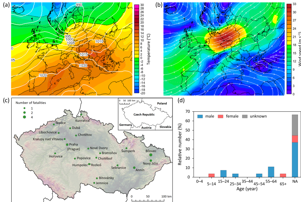
Figure 9. The windstorm of 7 December 1868 in the Czech Lands: (a) sea level pressure (hPa), air temperature and (b) wind speed at the 850 hPa level at 12:00 UTC (Wetterzentrale, 2026); (c) municipalities with fatalities; (d) distribution of fatalities according to sex and age.
