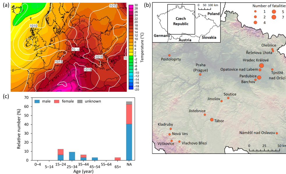
Figure 10. The convective storm of 4 July 1929 in the Czech Lands: (a) sea level pressure (hPa) and air temperature at the 850 hPa level at 18:00 UTC (Wetterzentrale, 2026); (b) municipalities with fatalities; (c) distribution of fatalities according to sex and age.
