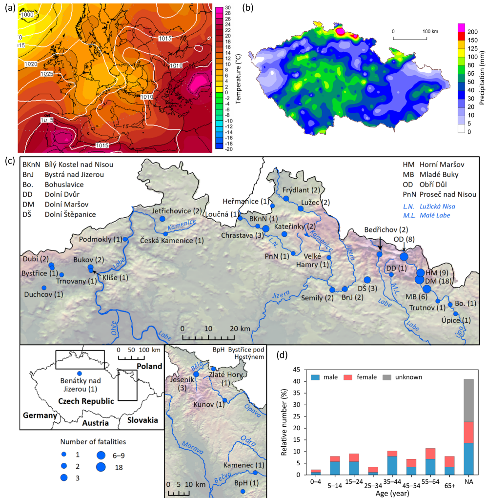
Figure 6. The flood of 30–31 July 1897 in the Czech Lands: (a) sea level pressure (hPa) and air temperature at the 850 hPa level on 29 July at 18:00 UTC (Wetterzentrale, 2026); (b) daily precipitation totals over the Czech Lands on 29 July; (c) municipalities with the number of fatalities; (d) distribution of fatalities according to sex and age.
