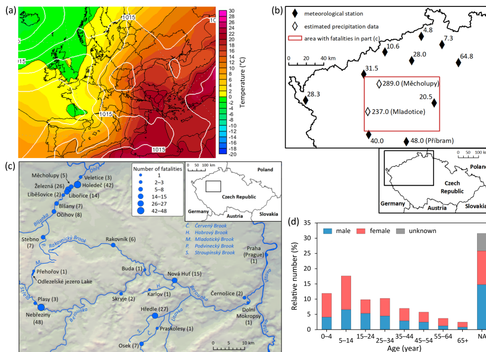
Figure 3. The flash flood of 25–26 May 1872 in western Bohemia: (a) sea level pressure (hPa) and air temperature at the 850 hPa level on 25 May at 12:00 UTC (Wetterzentrale, 2026); (b) daily precipitation totals (mm) on 25 May; (c) municipalities with the number of fatalities according to Bernat (1872); (d) distribution of fatalities according to sex and age.
