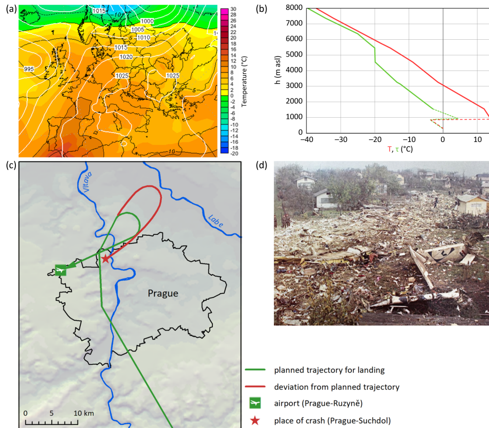
Figure 15. The air crash in fog of 30 October 1975 in Prague: (a) sea level pressure (hPa) and air temperature at the 850 hPa level at 06:00 UTC (Wetterzentrale, 2026); (b) vertical profile of the air temperature ( T ) and the dew point ( \tau ) at the Prague-Libuš station at 06:00 UTC – the reconstruction of both elements in the boundary layer using the dew point value at 12:00 UTC is shown by the dashed line (source: Integrated Global Radiosonde Archive, NOAA, https://www.ncei.noaa.gov/data/integrated-global-radiosonde-archive , last access: 16 December 2025); (c) planned trajectory of the plane for landing and the actual trajectory before the crash (Krupka, 2020); (d) place of the air crash in the cottage colony (photo: Národní archiv, Fond Úřadu pro civilní letectví – letecké nehody, in Poláček and Švec, 2024).
