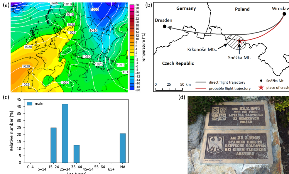
Figure 13. The air crash at “Sluneční jáma” in the Krkonoše Mts. on 23 February 1945: (a) sea level pressure (hPa) and air temperature at the 850 hPa level at 00:00 UTC (Wetterzentrale, 2026); (b) the scheduled flight lane and place of crash; (c) distribution of fatalities according to sex and age; (d) the memorial plaque with the inscription: “On 23 February 1945, 23 German soldiers died here in the fall of a plane” (source: Mapy.com – Mapy, 2025b).
