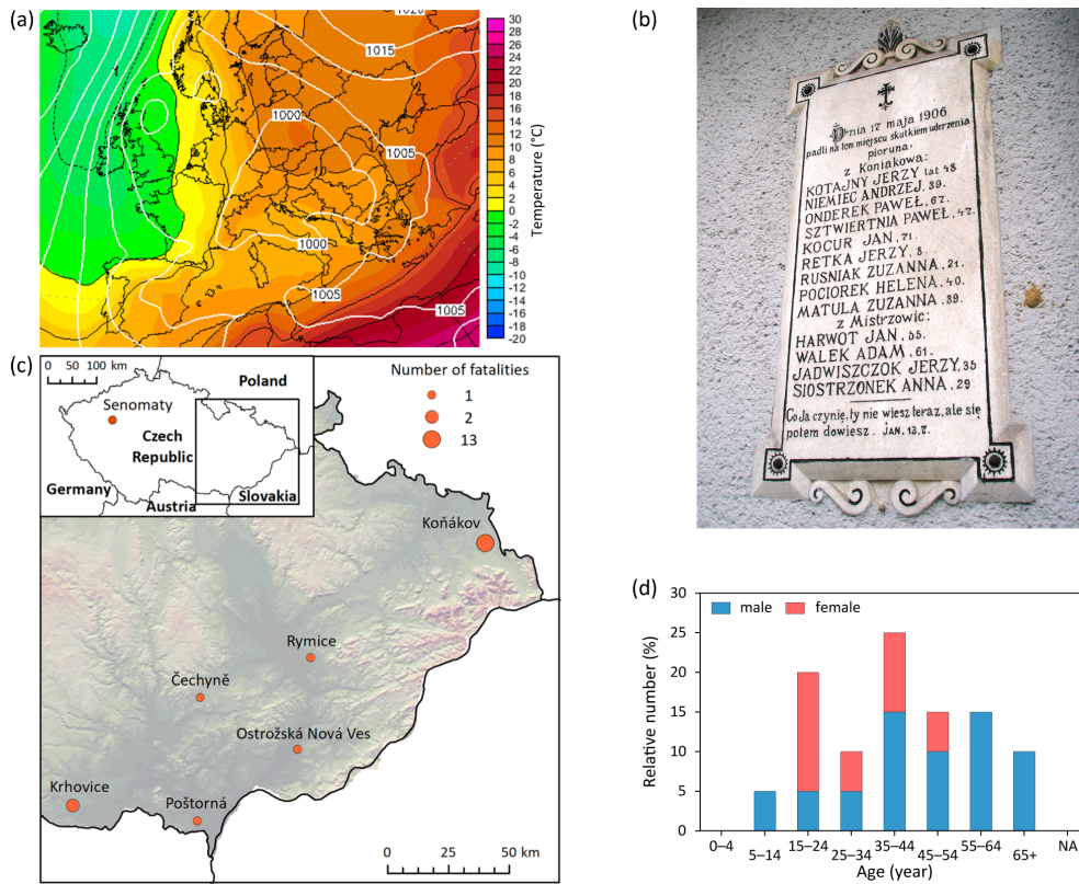
Figure 11. The thunderstorms of 17 May 1906 in the Czech Lands: (a) sea level pressure (hPa) and air temperature at the 850 hPa level at 12:00 UTC (Wetterzentrale, 2026); (b) memorial plaque of 13 lightning fatalities at the Koňákov cemetery (Qasinka, 2009); (c) municipalities with fatalities; (d) distribution of fatalities according to sex and age.
