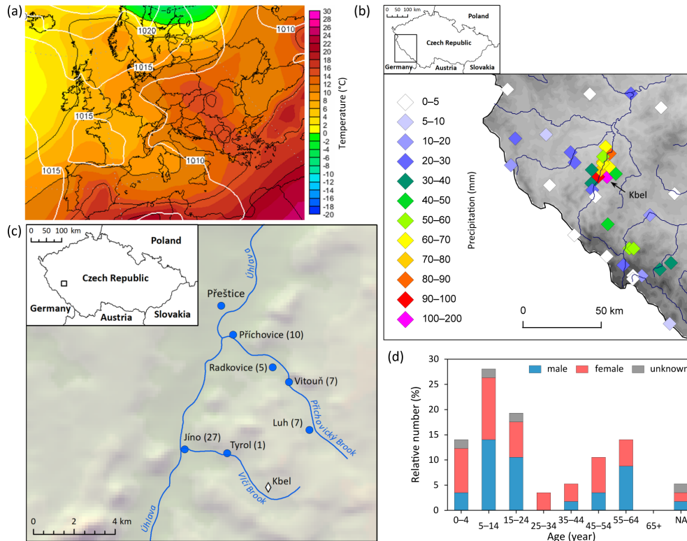
Figure 4. The flash flood of 17 May 1889 in the Přeštice region: (a) sea level pressure (hPa) and air temperature at the 850 hPa level on 16 May at 18:00 UTC (Wetterzentrale, 2026); (b) daily precipitation totals on 16 May; (c) municipalities with the number of fatalities; (d) distribution of fatalities according to sex and age.
