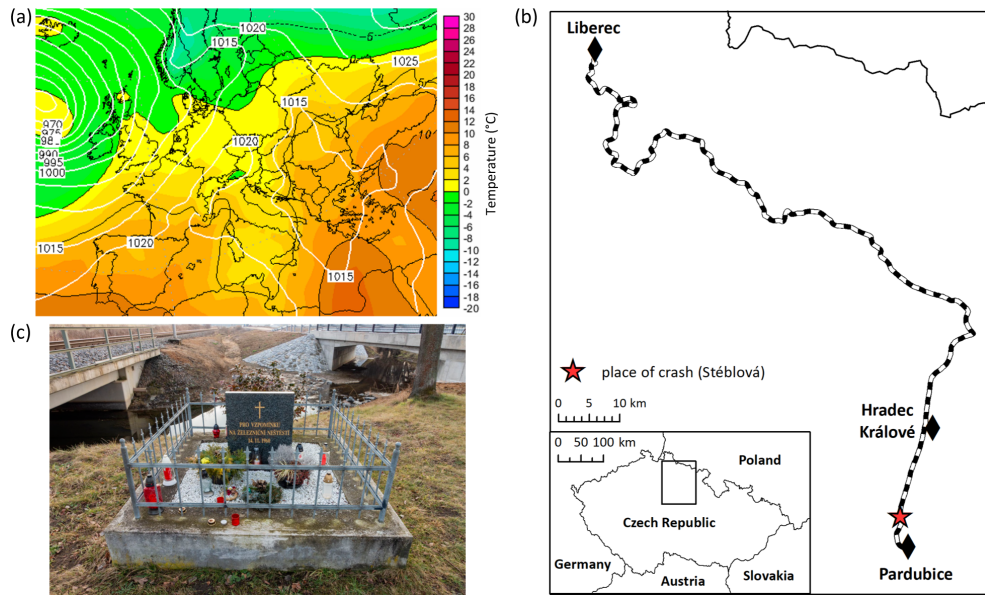
Figure 14. The train accident of 14 November 1960 near Stéblová: (a) sea level pressure (hPa) and temperature at the 850 hPa level at 18:00 UTC (Wetterzentrale, 2026); (b) geographic situation; (c) memorial to victims of the accident near Stéblová (source: Mapy.com – Mapy, 2025d).
