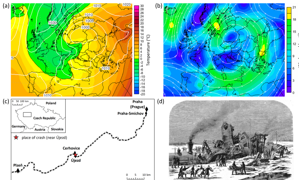
Figure 12. A tragic train crash in Újezd at Cerhovice on 10 November 1868: (a) sea level pressure (hPa), air temperature and (b) wind speed at the 850 hPa level at 00:00 UTC (Wetterzentrale, 2026); (c) geographic situation of train crash; (d) drawing of the crash by F. Chalupa from Světlozor (20 November 1868, p. 443).
