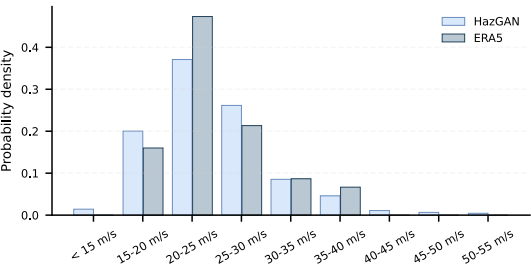
(c) Gaussian
