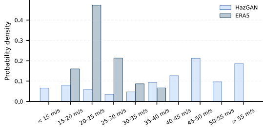
(b) Uniform
