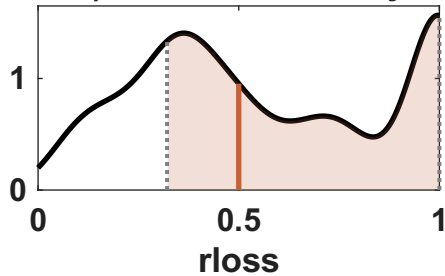
d) Predictive density
