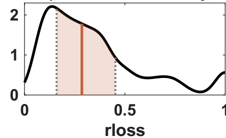
f) Predictive density
