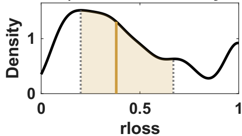
b) Predictive density
