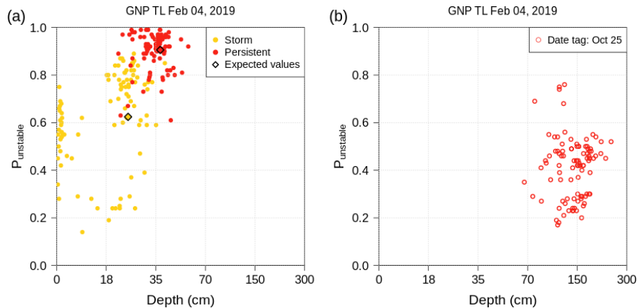
Figure 4. Numerical hazard charts derived from snowpack simulations that are similar to the ones produced by forecasters (Fig. 1). As described in the text, the data can be subset by avalanche problem types and date tags such that each data point corresponds to one grid point location showing the weakest instability ( p_{\text{unstable}} ) and the relevant failure depth for the given subset. (a) Storm snow and persistent weak layer problems and (b) the subset for a specific date tag (25 October, the green layer close to the ground in Fig. 3).
