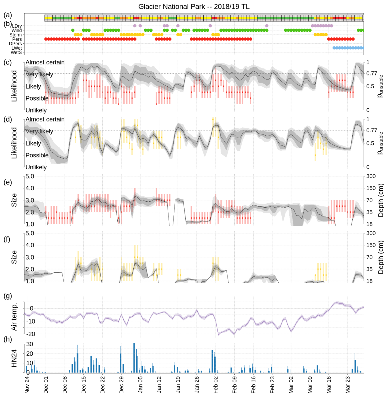
Figure 5. Season summary 2018/2019 of human hazard assessments and modeled hazard characteristics for Glacier National Park. (a) Reported danger rating and (b) avalanche problems at treeline elevation. (c, d) Reported likelihood of avalanches from persistent (red) and storm slab avalanche problems (yellow). In addition, modeled distribution of p_{\text{unstable}} with the envelope of the 10th–90th percentiles (light gray shading), the interquartile range (dark gray shading), and the expected value (black line). (e, f) Analogous to the previous two panels but showing the reported size of avalanches and the modeled failure depth. (g) Modeled interquartile range and median air temperature in units of degrees Celsius. (h) Modeled median height of new snow within 24 h in units of centimeters (HN24).
