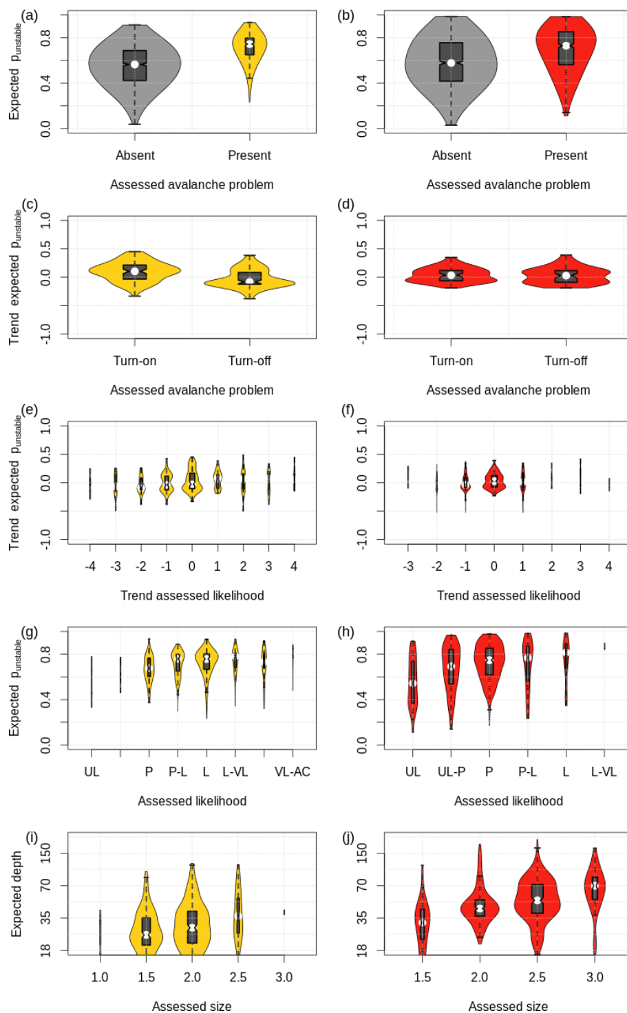
Figure 8. Multi-season distributions of numerical hazard characteristics grouped by categorical assessments of human forecasters for (a, c, e, g, i) storm snow problems and (b, d, f, h, j) persistent weak layer problems.
