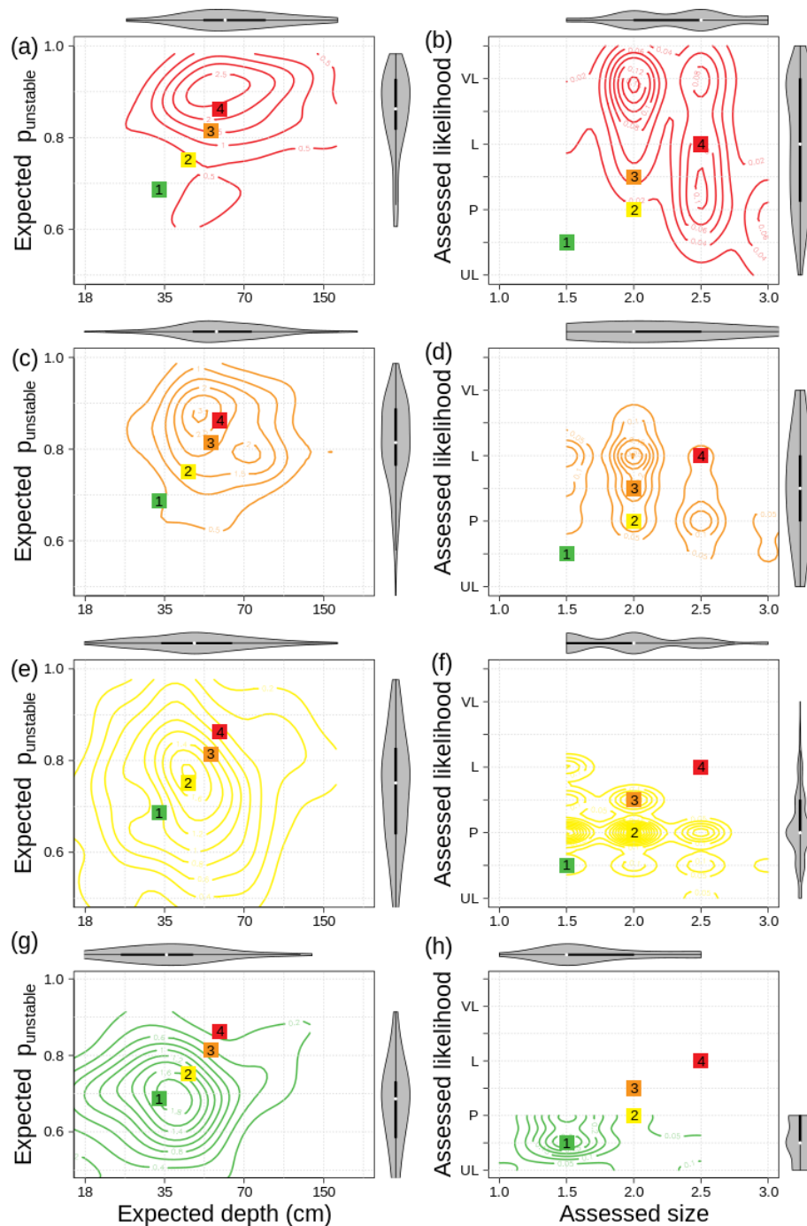
Figure 7. (a, c, e, g) Contour maps of the numerical hazard chart and (b, d, f, h) the human assessment hazard chart stratified by different danger ratings from human assessments. The colored square labels highlight the median values of the contour maps and are identical within the left and right columns of the panels. The violins show the marginal distributions of the contours. While the expected p_{\text{unstable}} and the expected depth represent continuous numbers, the assessed likelihood and size are expressed on five-level ordinal scales with half steps, which causes the contours to appear binned around the grid intersections.
