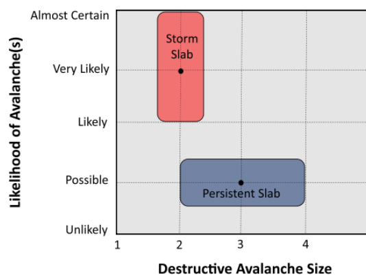
Figure 1. The hazard chart as part of the CMAH allows us to quickly understand the severity of distinct avalanche problems. Taken from Statham et al. (2018a).
