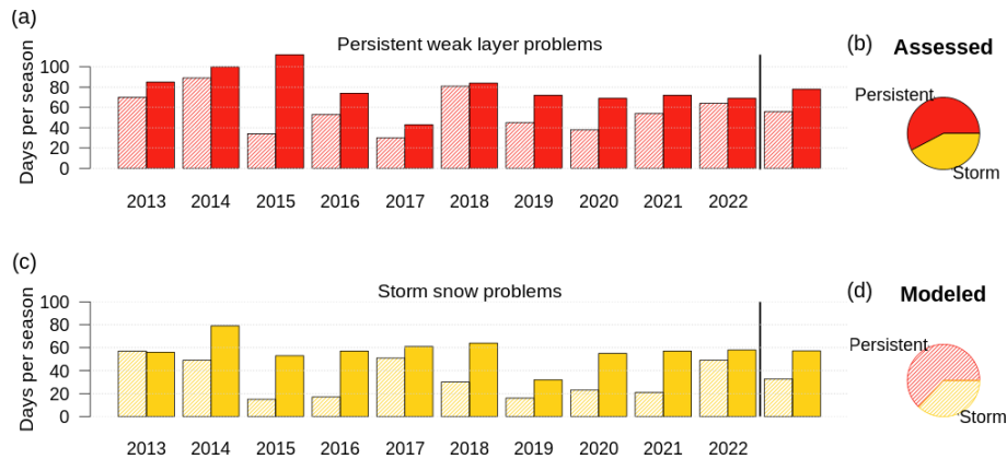
Figure 6. (a, c) The number of days per season with assessed and modeled persistent weak layer and storm snow problems in Glacier National Park. Solid colors refer to human assessments and hatched colors to model results. (b, d) The relative frequency of assessed and modeled problems. A threshold of the average p_{\text{unstable}} \geq 0.77 was used to label a problem as modeled.
