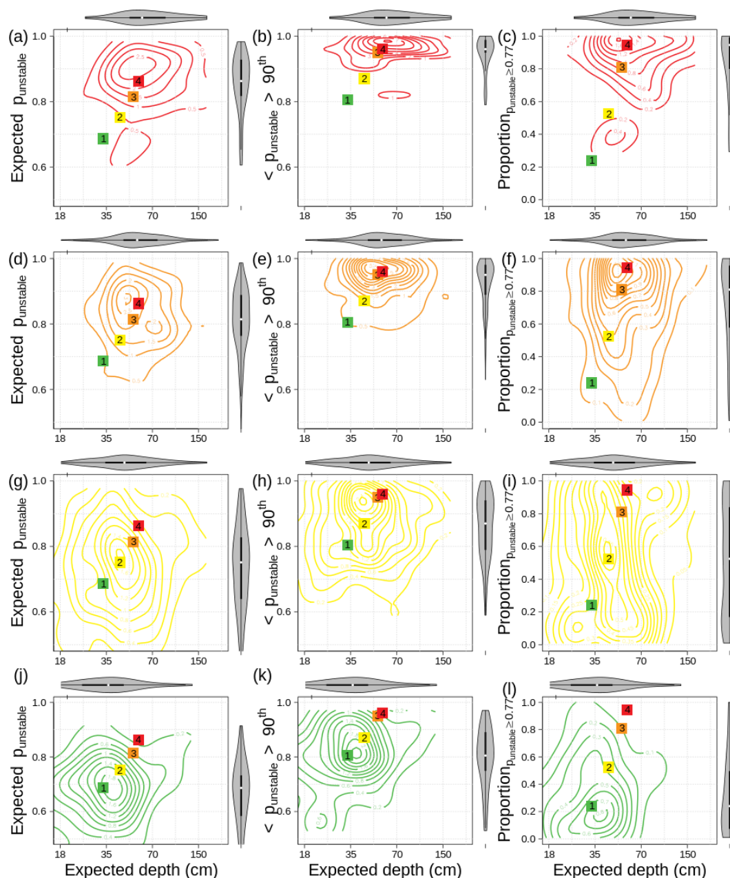
Figure A1. Contour maps of the numerical hazard chart, using the expected p_{\text{unstable}} (i.e., 50th percentile) as in Fig. 7a, c, e, and g (left column); the 90th percentile of p_{\text{unstable}} (middle column); and the proportion of unstable grid points with p_{\text{unstable}} \geq 0.77 (right column). The charts are stratified by their reported danger ratings from human assessments (different rows). The colored square labels highlight the median values of the contour maps and are identical within each column. The violins show the marginal distributions of the contours.
