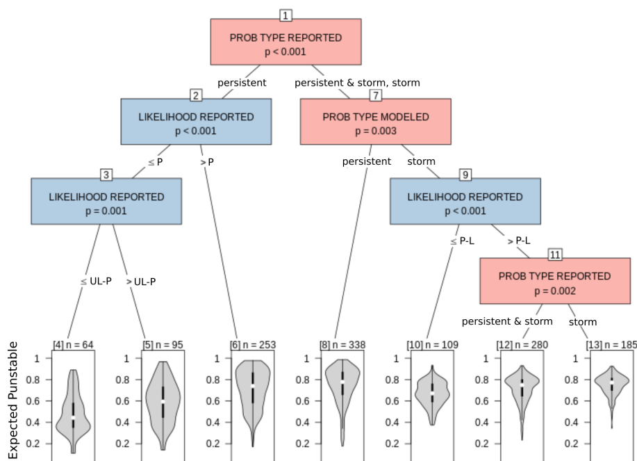
Figure 9. CTree for the expected p_{\text{unstable}} examining the interaction effects of explanatory variables extracted from human assessments.
