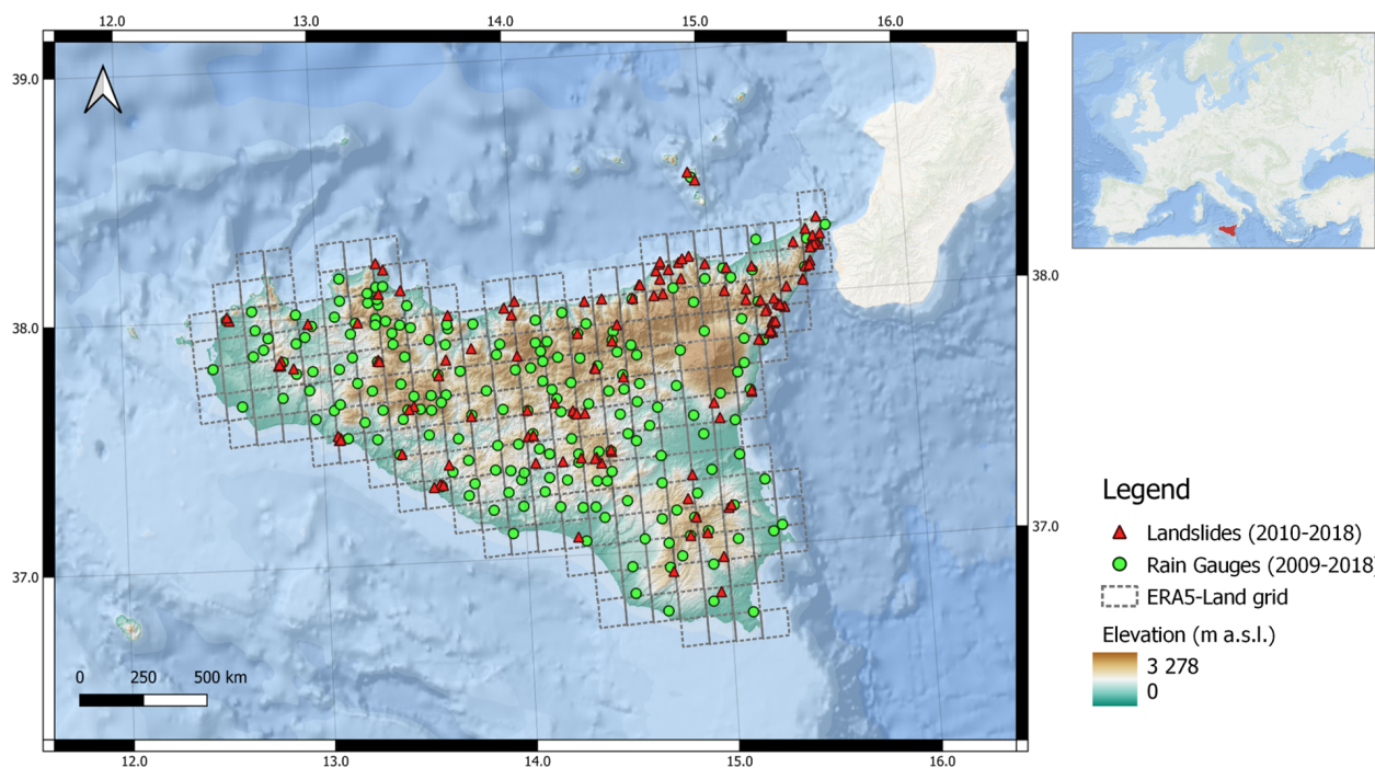
Figure 3. Study area map (credit to https://www.sitr.regione.sicilia.it/geoportale/mobile/search.html?q=dem , last access: 4 December 2025, and ESRI, 2020). Red triangles represent the locations of the occurred landslides in the study area from 2010 to 2018 and retrieved by the FraneItalia catalogue; green dots represent the locations of the 306 gauges installed in Sicily.
