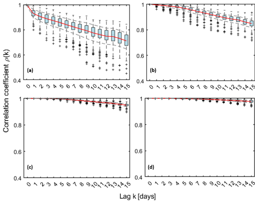
Figure 4. Conditional autocorrelation function for soil moisture at the four ERA5-Land depths (time lags from 1 to 15 d) (a) 0–7 cm; (b) 7–28 cm; (c) 28–100 cm; (d) 100–239 cm.
