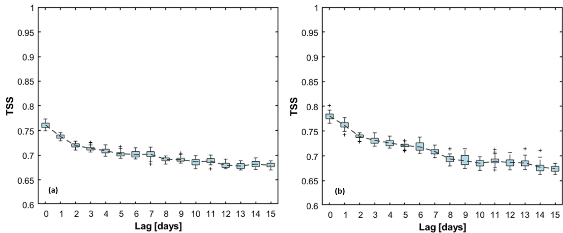
Figure 5. TSS values from 30 ANN training runs, with the dashed grey line representing the mean TSS across lag time. (a) Simulation set with rainfall duration ( D , [h]), rainfall depth ( E , [mm]) and soil moisture at the second-layer depth as input dataset; (b) Simulation set with rainfall duration ( D , [h]), rainfall depth ( E , [mm]) and soil moisture at all -layer depth as input dataset.
