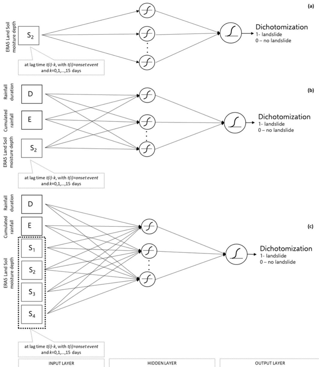
Figure 2. Sketch of the implemented ANN model. Soil moisture subscripts ( S ) indicate the soil layer (depth range) of the ERA5-Land reanalysis dataset. (a) Soil moisture in the 7–28 cm layer at increasing lags; (b) Soil moisture in the 7–28 cm layer at increasing lags together with cumulated rainfall and rainfall duration; (c) Multilayer soil moisture at increasing lags together with cumulated rainfall and rainfall duration. All variables are used as inputs to the ANN.
