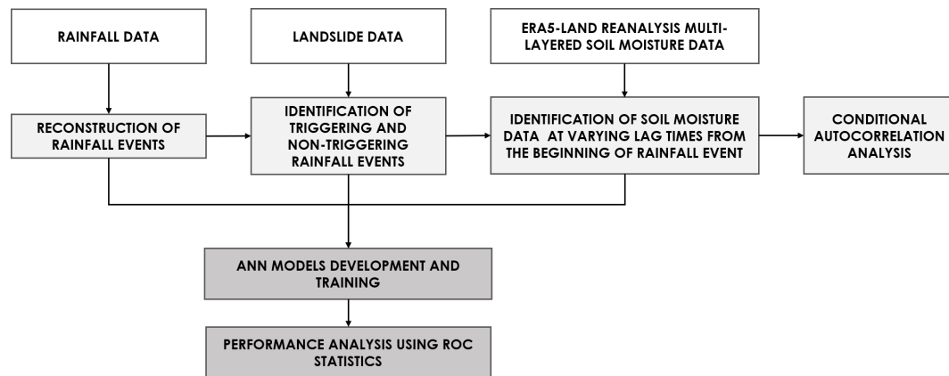
Figure 1. Scheme of the methodology applied to explore the potential use of delayed ERA5-Land soil moisture products for the identification of landslide triggering conditions.
