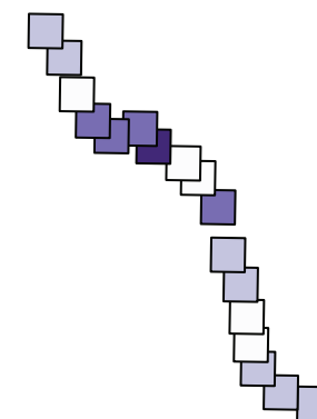
Precipitation
