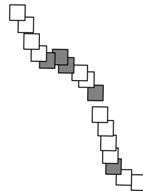
Landslides
