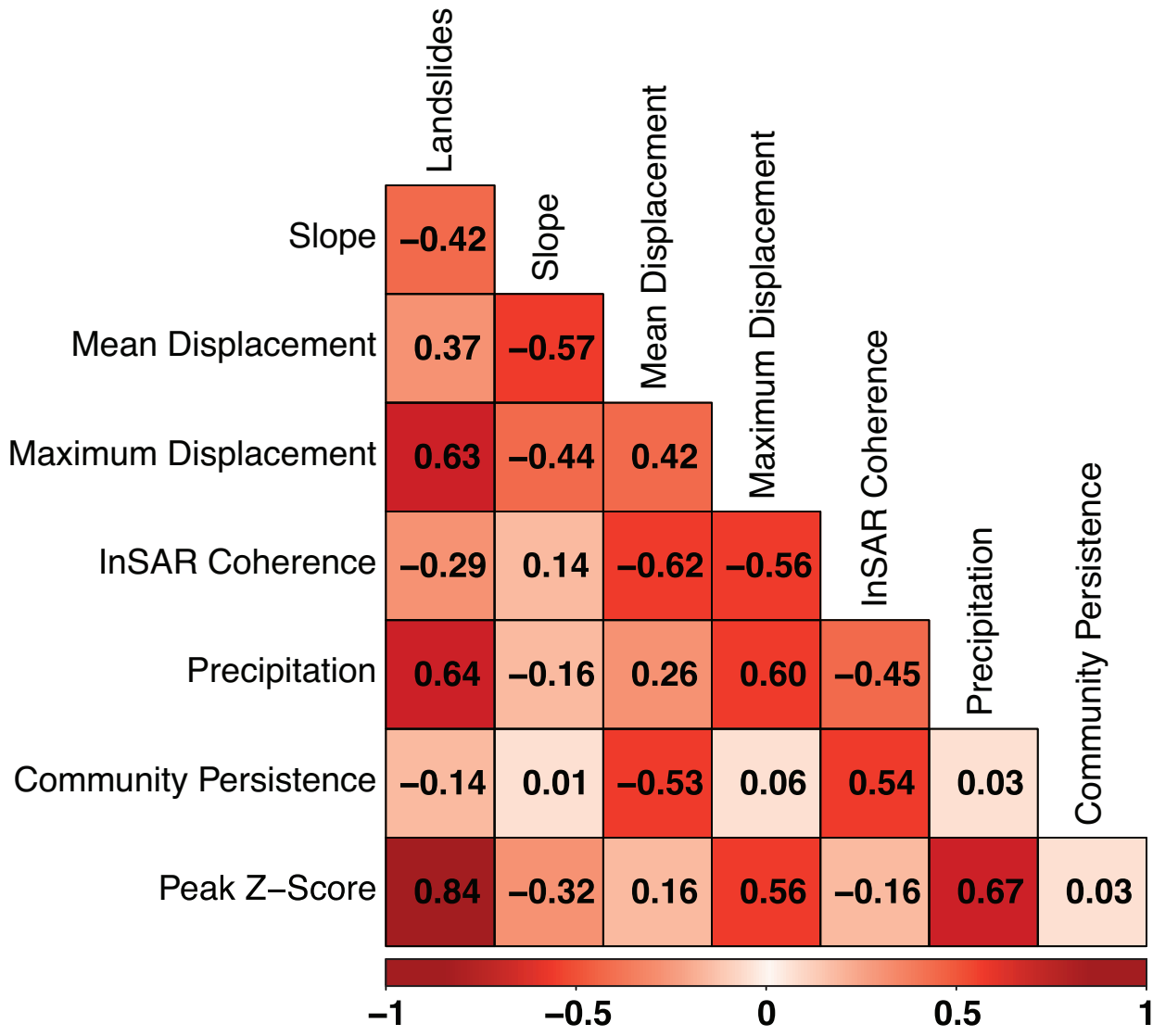
Landslides
