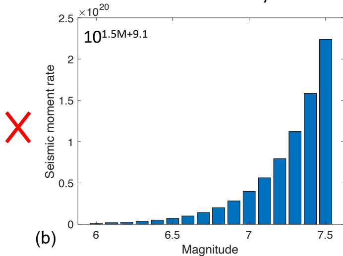
Seismic moment rate per magnitude – at the scale of the system
