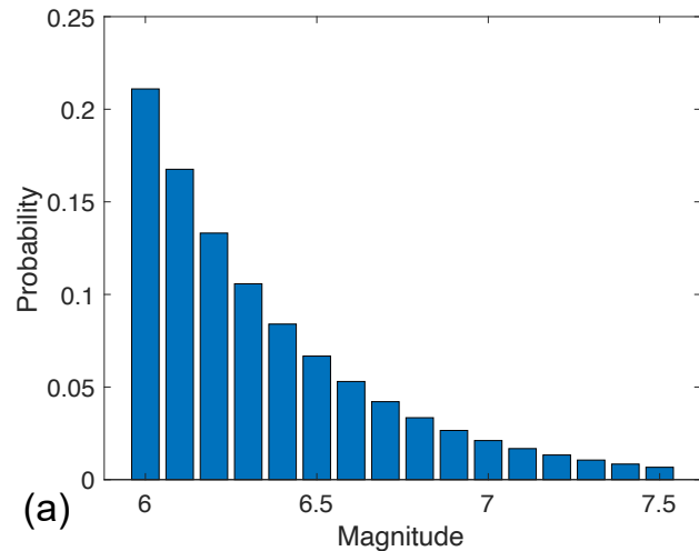
PDF of the Gutenberg Richter model – at the scale of the system
