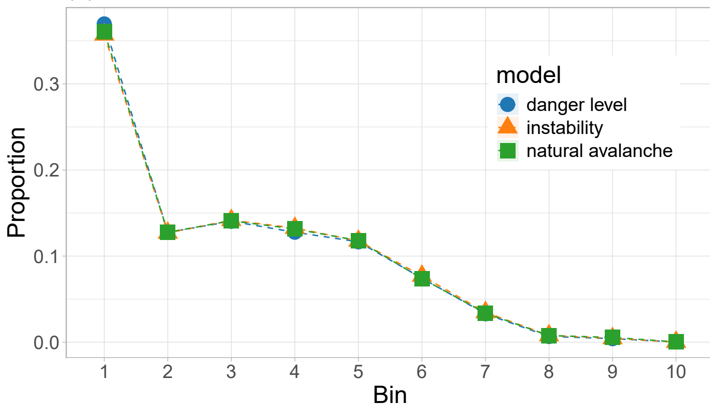
(c) Events (natural avalanches)
