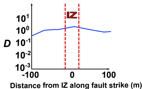
(b) Fault-parallel linear infrastructure
