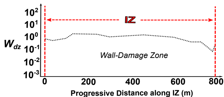
(c) Near-fault tip linear infrastructure
