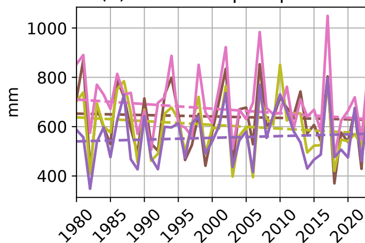
(e) Corrected precipitation
