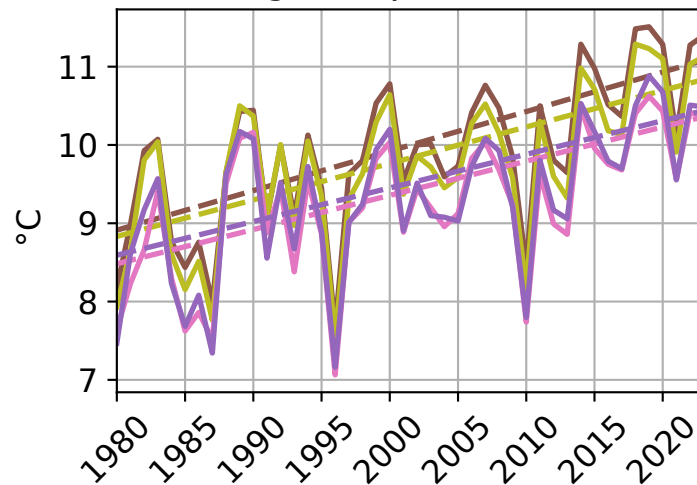
(b) Avg. temperature in 2 m
