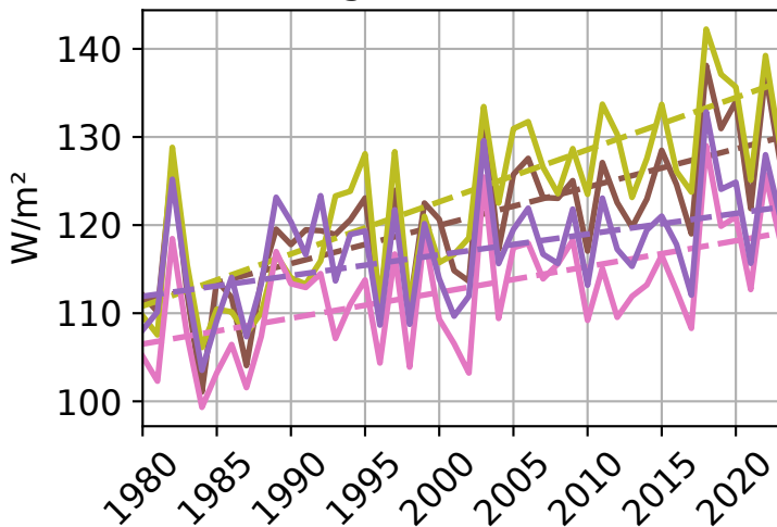
(a) Avg. solar irradiation
