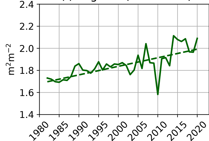
(f) Avg. LAI (state-wide)
