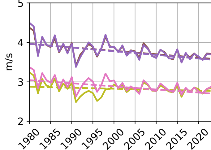
(c) Avg. wind speed
