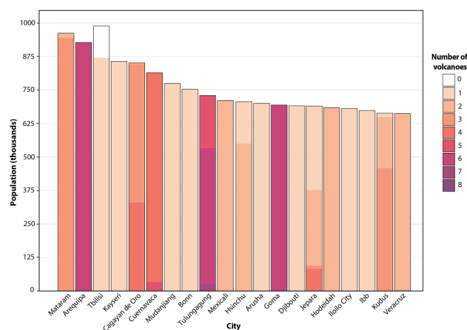
Figure A2. Top 20 cities with exposed populations below 1 million, coloured by the number of volcanoes for which a city lies within a 100 km radius.
