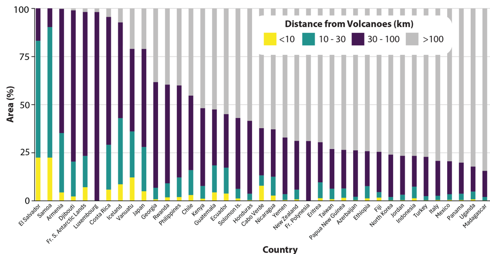
Figure A4. Top 40 countries with a total area of > 2000 km 2 ranked in order of their total land area exposed to volcanic hazards and coloured by the percentage of the area. Is. stands for islands, Fr. stands for French, and S. stands for southern. Land area from Natural Earth (2023).
