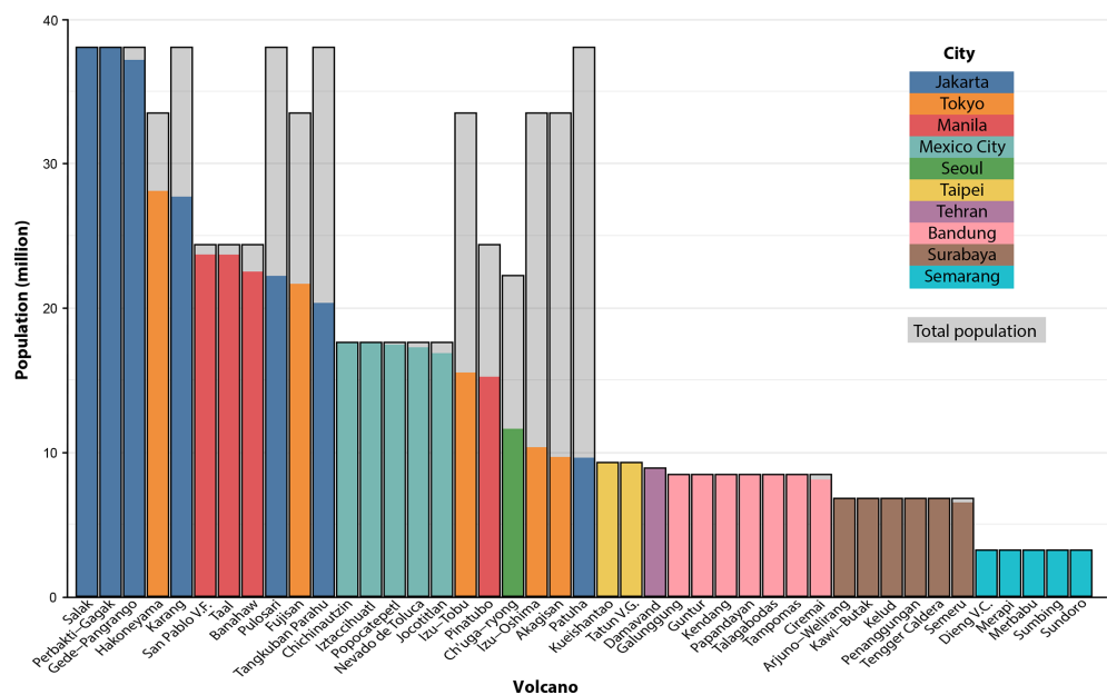
Figure A3. City populations exposed to individual volcanoes within 100 km, ranked by the dominant city. Bars are coloured by the dominant city’s exposed population. V.F. stands for Volcanic Field, V.G. stands for Volcanic Group, and V.C. stands for Volcanic Complex.
