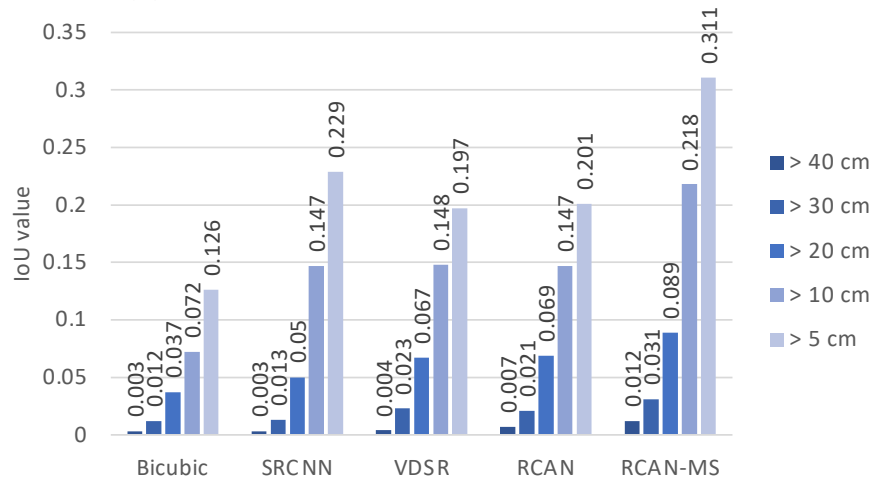
(b) Dataset 1. IoU Evaluation of Flood Area
