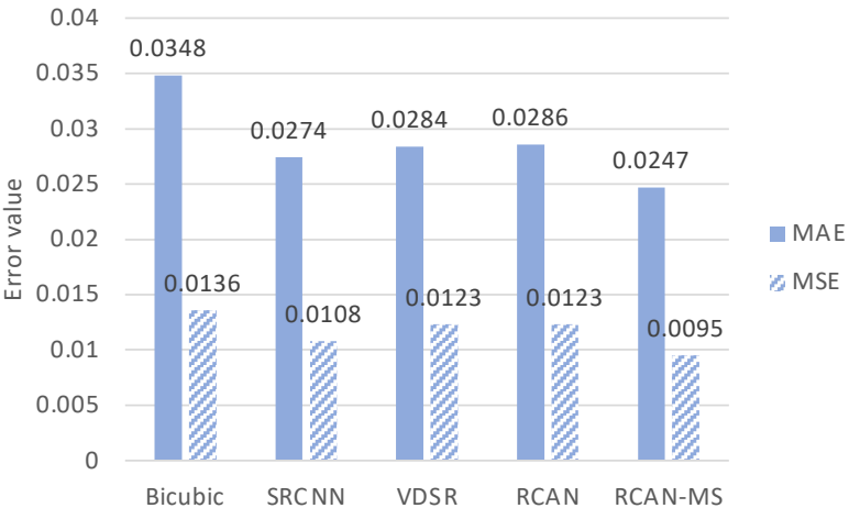
(a) Dataset 1. Flood Depth
