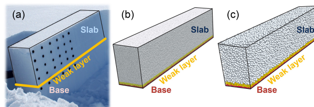
Figure 1. (a) Experimental propagation saw test (PST; photo: Jürg Schweizer). The black dots are markers used to measure slab deformation (particle tracking). (b) Material point method PST simulation. (c) Discrete element method PST simulation, length 2 m.
