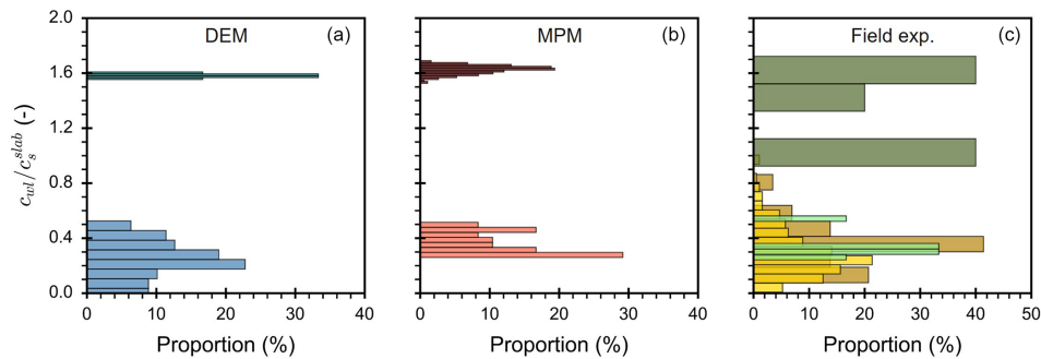
Figure 2. Compilation of crack propagation speeds (normalized to slab shear wave speed), relative frequency shown. (a) DEM simulations (blue \psi = 0^\circ , teal \psi = 30\text{--}45^\circ ). (b) MPM simulations (orange \psi = 0\text{--}20^\circ , maroon \psi = 25\text{--}50^\circ ). (c) Field measurements, either extracted from short PSTs (yellow \psi < 30^\circ , dark yellow \psi \geq 30^\circ ) or derived from avalanche video sequences (light green cross-slope and dark green down-slope crack propagation speeds).
