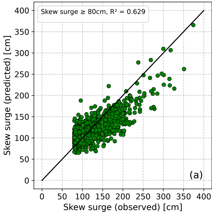
Ridge regression
