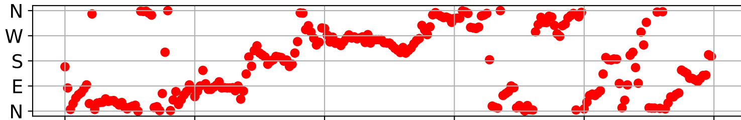
New Snow
