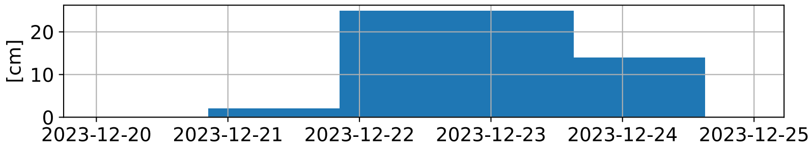
New Snow
