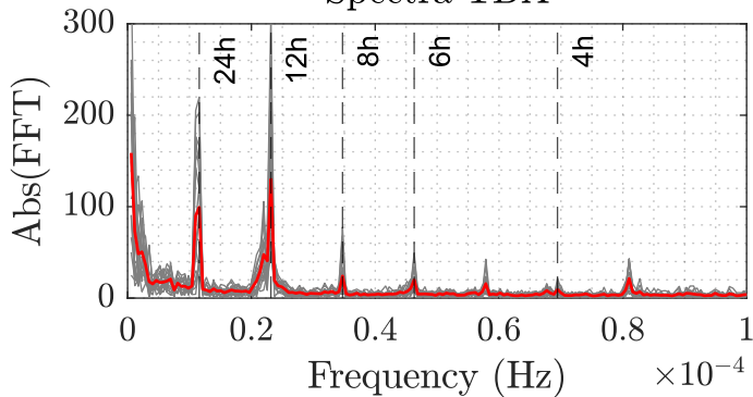
Spectra TDA
