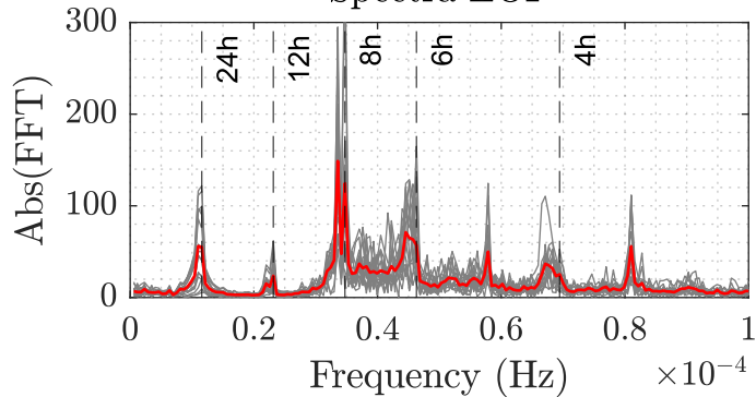
Spectra FIF
