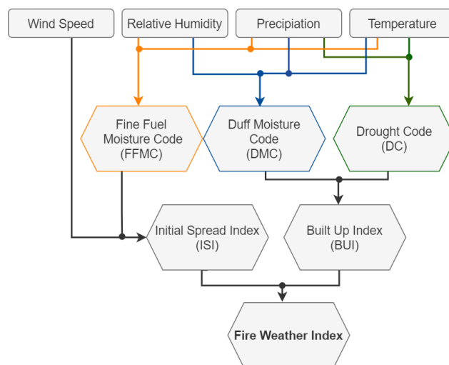
Figure 2. The Canadian Forest Fire Weather Index System, its input variables, and its intermediate indices. Fuel moisture codes (FFMC, DMC, and DC) capture the antecedent moisture conditions of the organic matter. Fire behavior codes (ISI, BUI, and FWI) describe the potential spread and intensity of the fire (modified from van Wagner, 1987).
