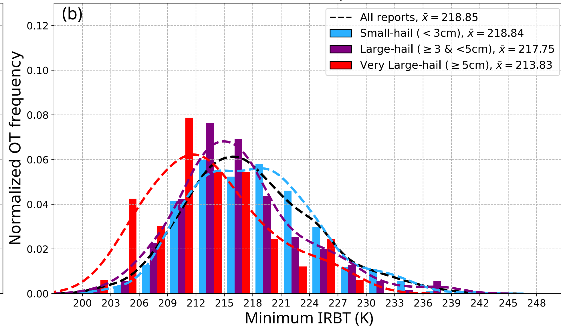
Misses (771 reports)
