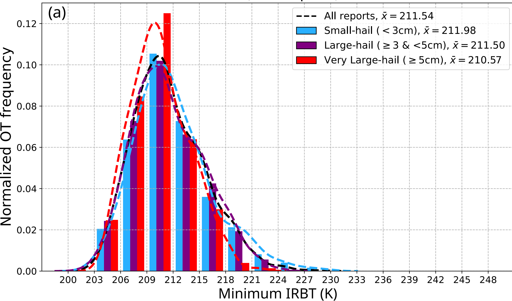
Hits (1478 reports)
