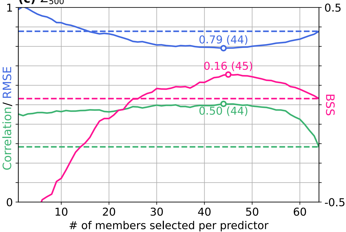
(c) Z_{500}
