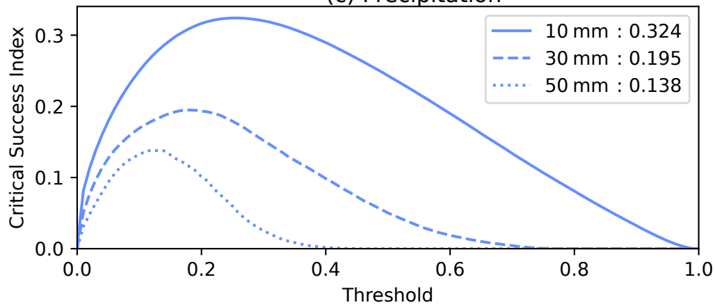
(c) Precipitation
