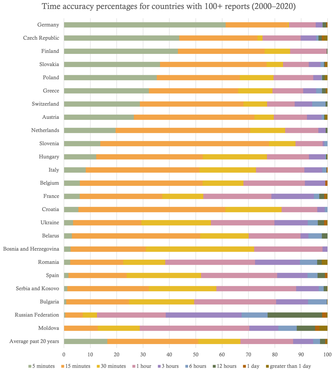
Figure 12. Horizontal bar charts of the time accuracy for countries with 100 or more reports (%) for 2000–2020.
