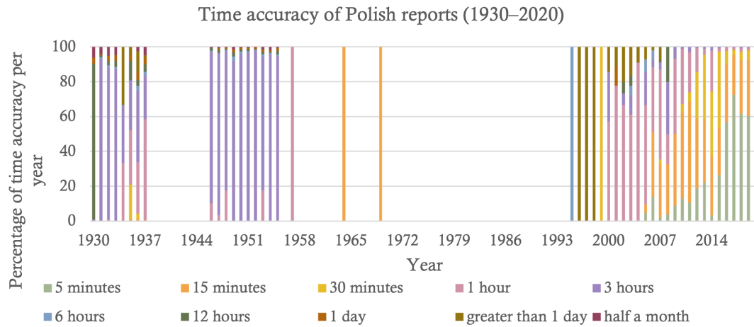
Figure 17. Time series of bar charts of the annual distributions of the time accuracy of reports for Poland (%) for 1930–2020.
