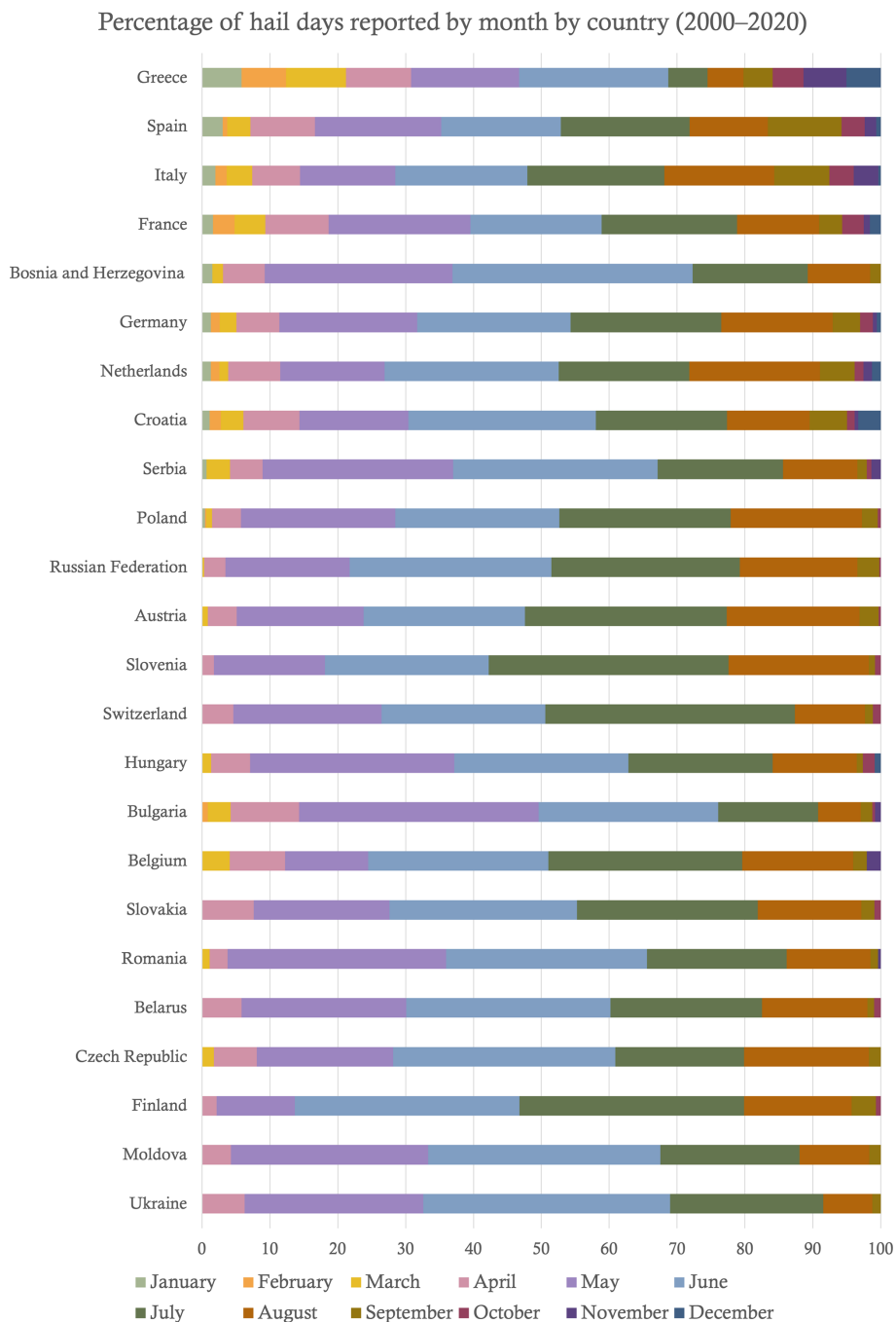
Figure 4. Horizontal bar charts of the monthly distributions of large-hail reports (%) for countries with 100 or more reports for 2000–2020.
