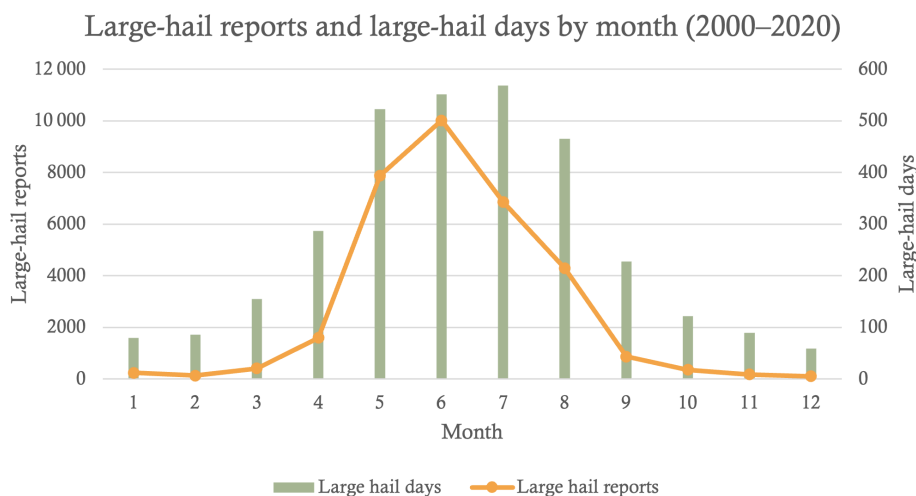
Figure 3. Combined line graph and bar chart of the total monthly numbers of large-hail reports (orange line) and large-hail days (green bars) across Europe for 2000–2020. These quantities are not divided by the number of years because of the incomplete data for the year 2020.
