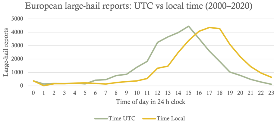
Figure 5. Distribution of the hourly time of large-hail reports across Europe in UTC (green line) and local time (orange line) for 2000–2020. Reports are associated with the starting hour (i.e. a report at 15:15 UTC would be placed in the 15:00 UTC bin).
