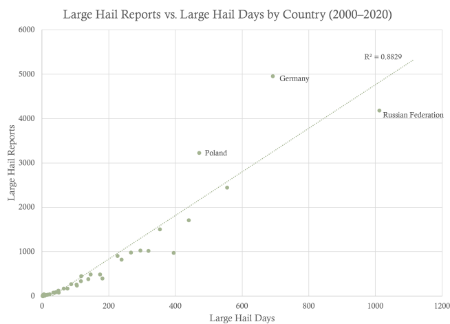
Figure 13. Scatterplot of the total number of large-hail reports versus large-hail days by country for 2000–2020.
