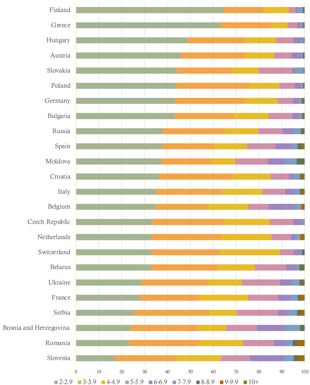
Figure 15. Horizontal bar charts of the size distribution of large hail for countries with 100 or more reports (%) for 2000–2020.
