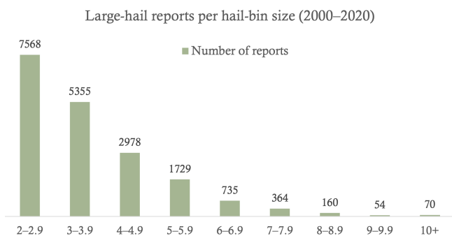
Figure 8. Bar chart of the number of large-hail reports across Europe by maximum diameter in 1 cm bins for 2000–2020.
