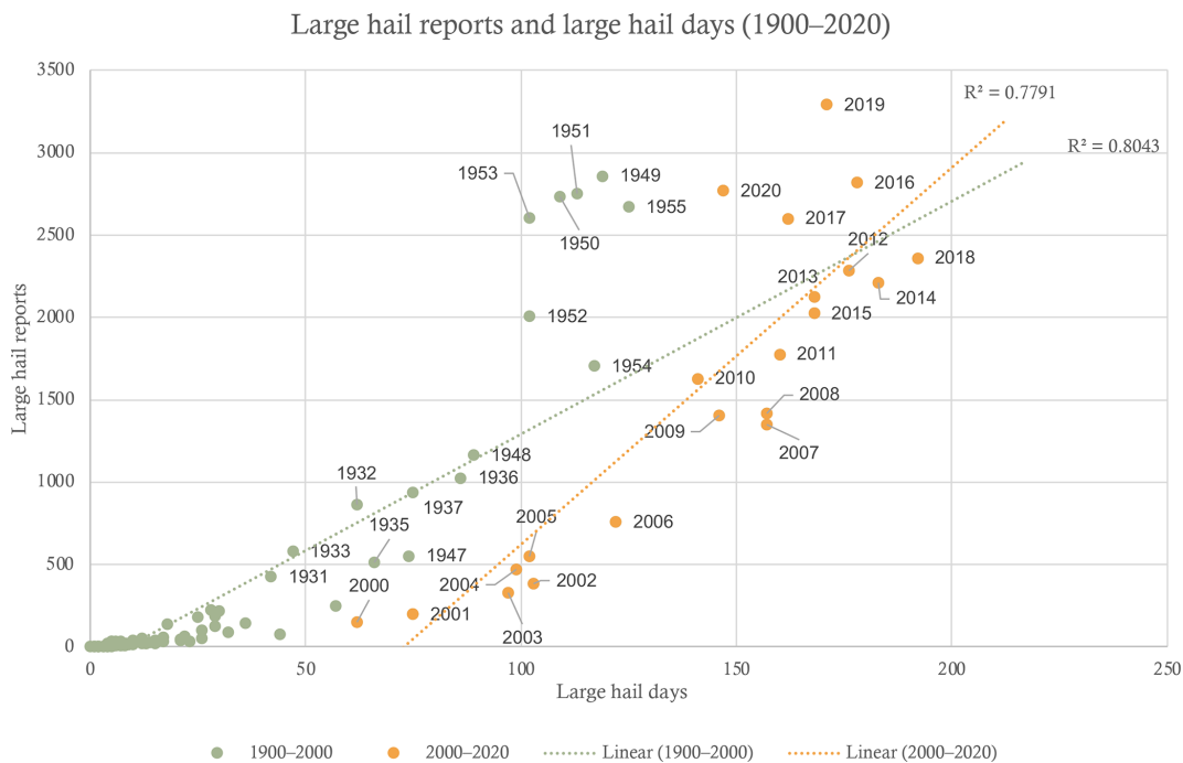
Figure 2. Scatterplot of the annual number of large-hail days versus annual number of large-hail reports across Europe for 1900–2000 (green dots) and 2000–2020 (orange dots), with corresponding linear regression lines. These quantities are not divided by the number of years because of the incomplete data for the year 2020.
