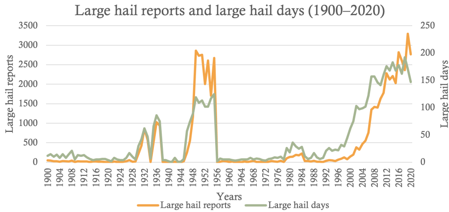
Figure 1. Time series of annual numbers of large-hail reports (orange line) and large-hail days (green line) across Europe for 1900–2020.
