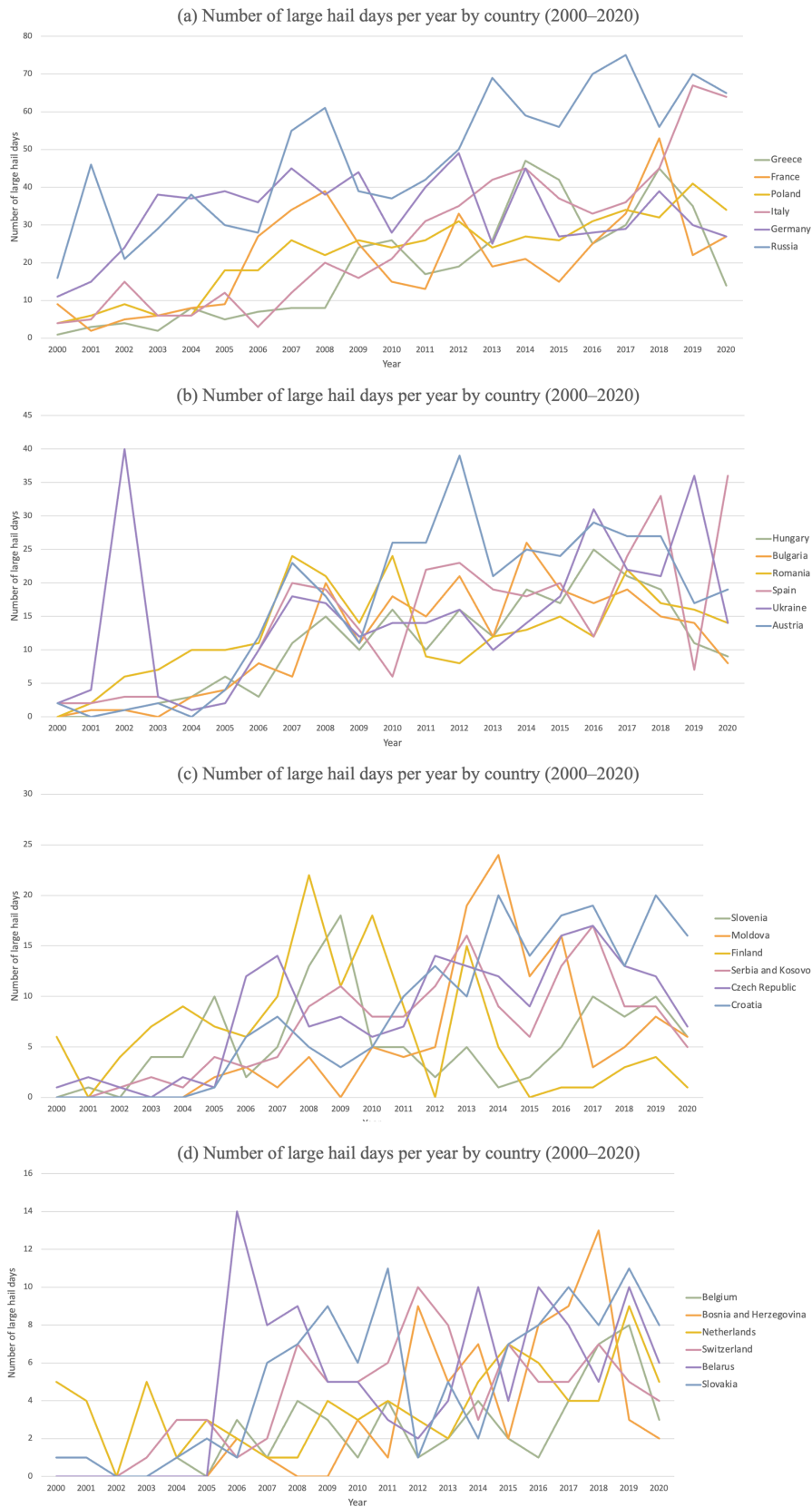
Figure 14. Line graph of large-hail days per country for countries with 100+ reports for 2000–2020: (a) top six countries, (b) upper-middle six countries, (c) lower-middle six countries, and (d) bottom six countries.
