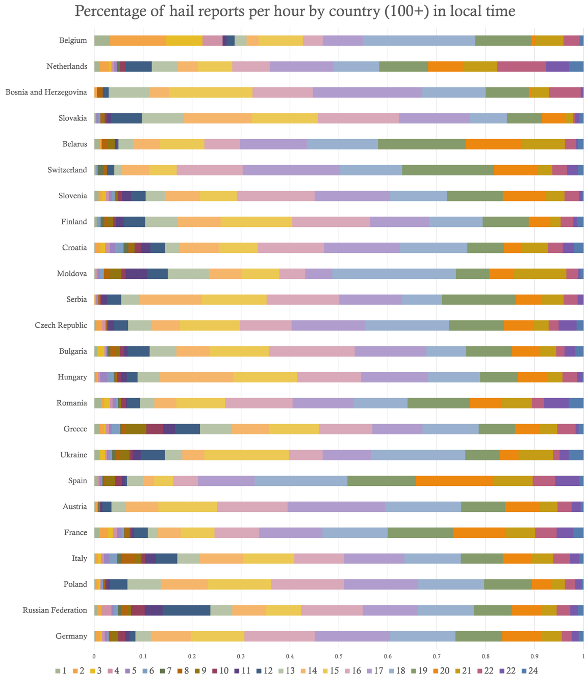
Figure 7. Horizontal bar charts of the hourly distributions of large-hail reports (percentage divided by 100) for countries with 100 or more reports for 2000–2020.
