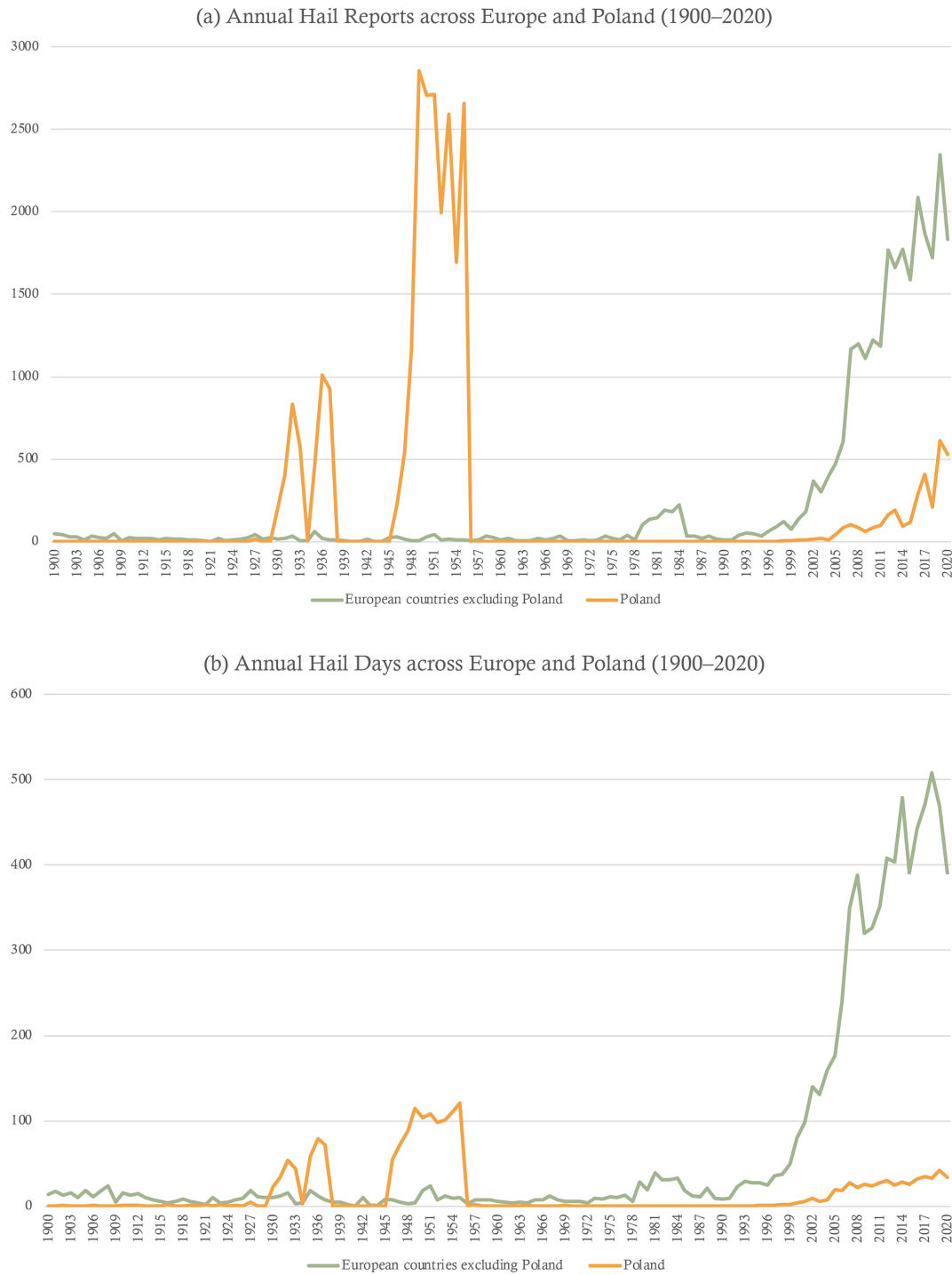
Figure 16. Time series of annual numbers for 1900–2020 of (a) large-hail reports for Europe (green line) and Poland (orange line) and (b) large-hail days for Europe (green line) and Poland (orange line).
