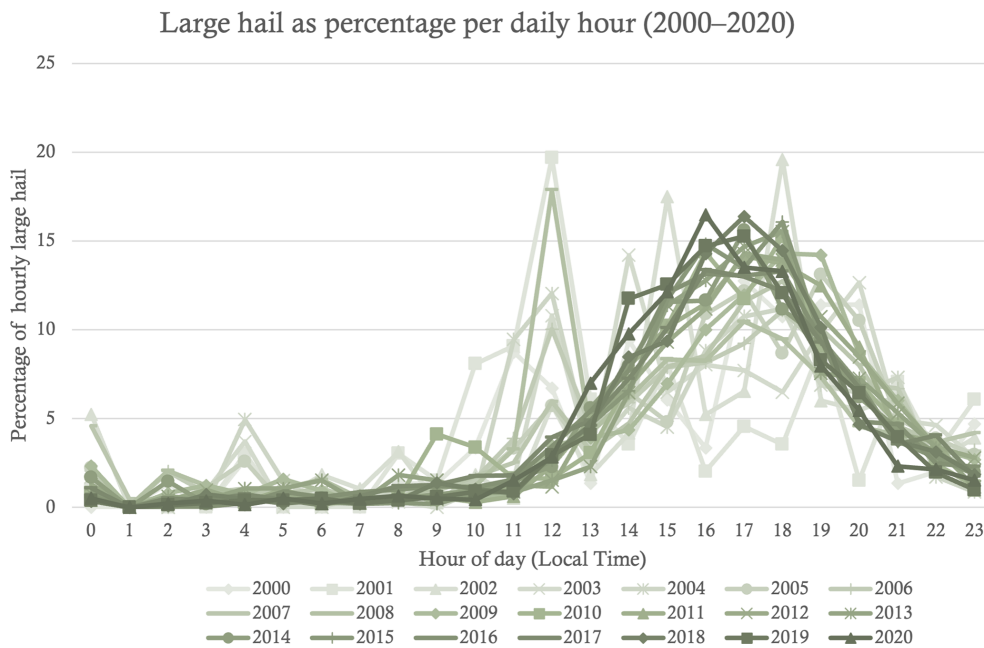
Figure 6. Hourly percentage of large hail in local time across Europe in local time for each year from 2000 to 2020.
