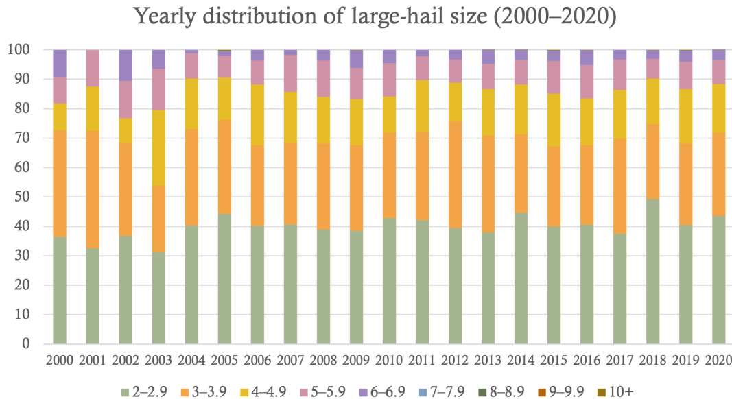
Figure 9. Time series of bar charts of the annual distributions of large-hail size across Europe in 1 cm diameter bins (%) for 2000–2020.
