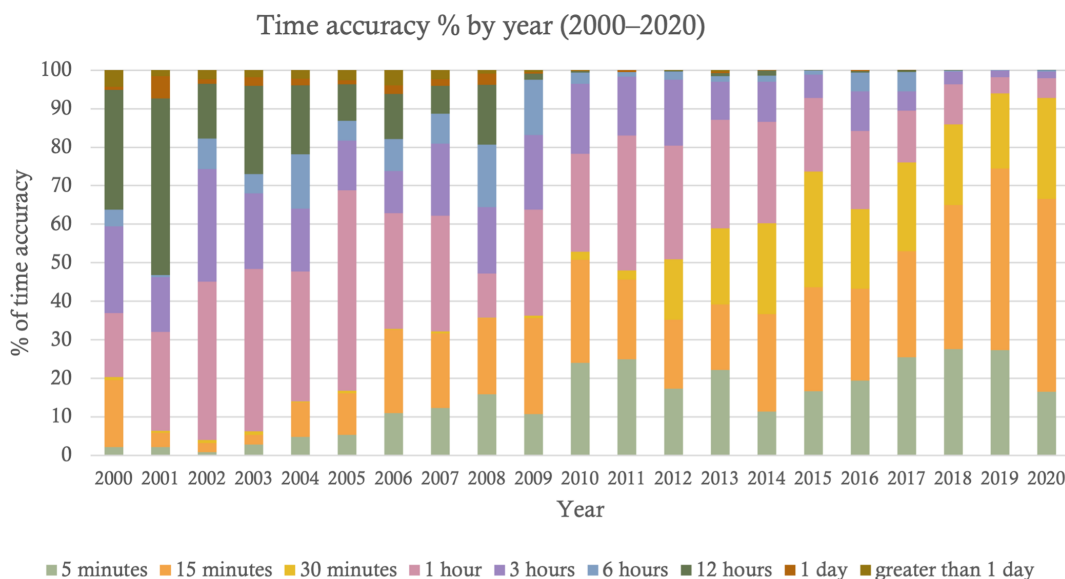
Figure 11. Time series of bar charts of the annual distributions of the time accuracy of reports across Europe (%) for 2000–2020.
