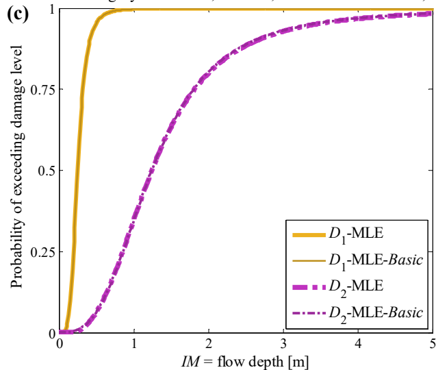
MLE-based fragility assessment, Model 2, Palu-Sulawesi Tsunami, Class 3
