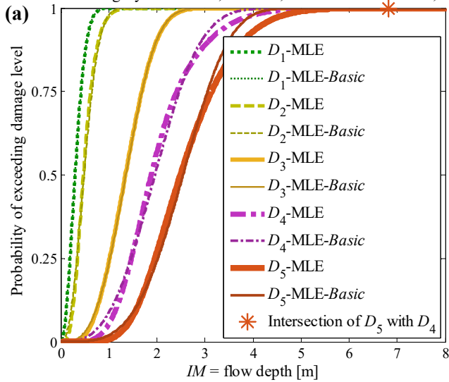
MLE-based fragility assessment, Model 1, Palu-Sulawesi Tsunami, Class 1
