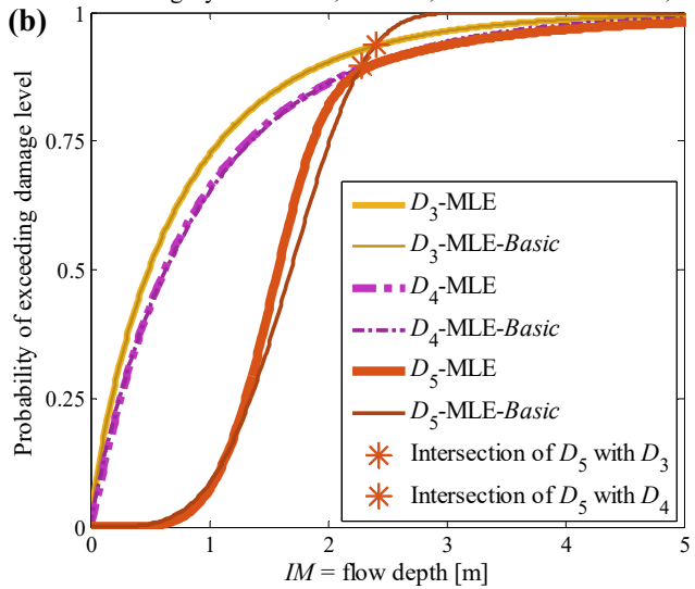
MLE-based fragility assessment, Model 3, Palu-Sulawesi Tsunami, Class 2
