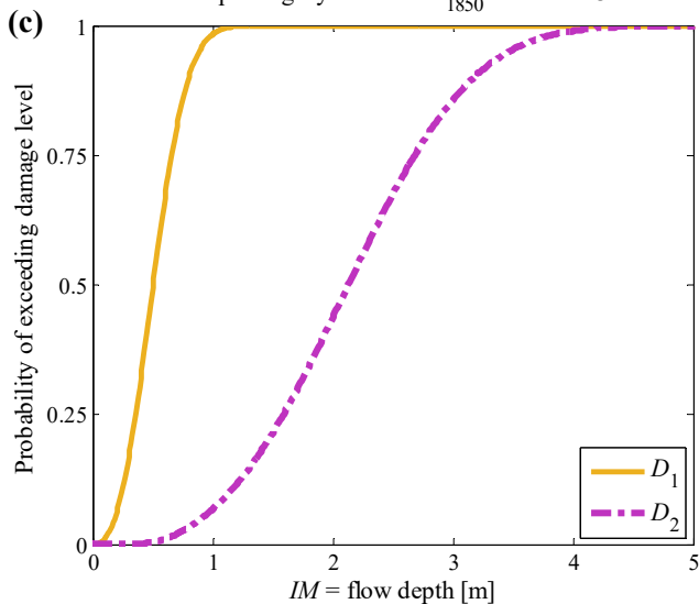
Sample fragility based on \theta_{1850} for Model 3
