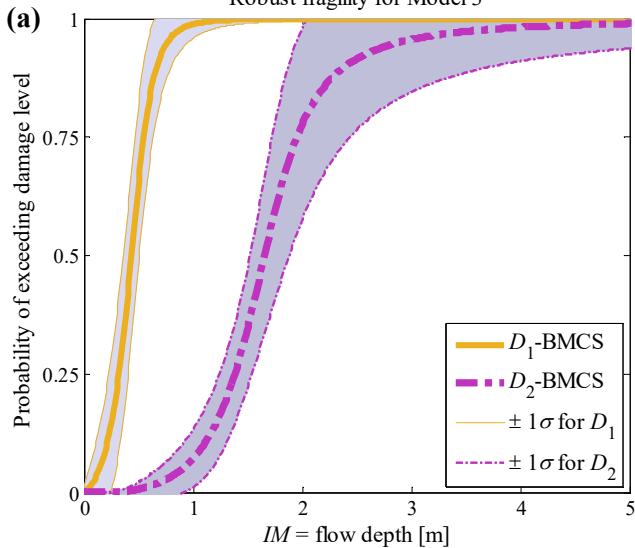
Robust fragility for Model 3
