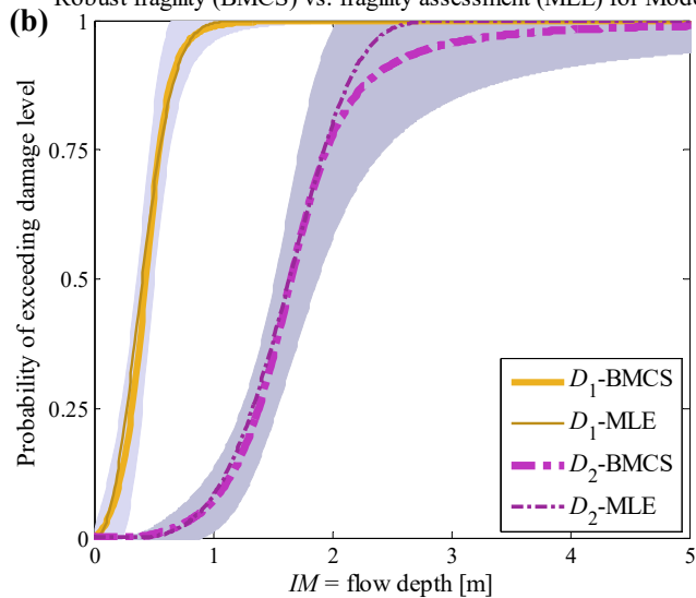
Robust fragility (BMCS) vs. fragility assessment (MLE) for Model 3
