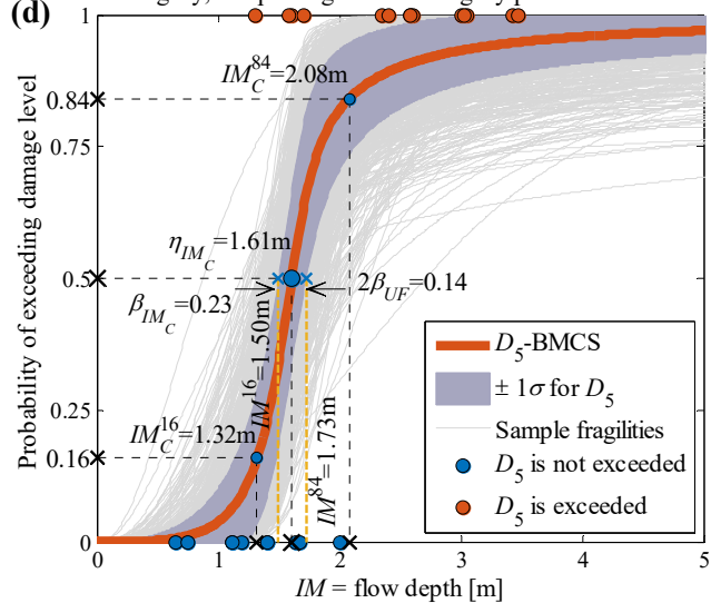
Robust fragility, sample fragilities and fragility parameters for Model 3
