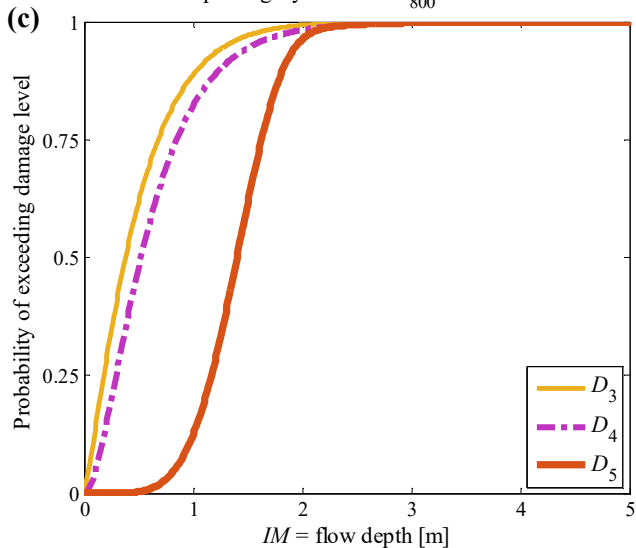
Sample fragility based on \theta_{800} for Model 3
