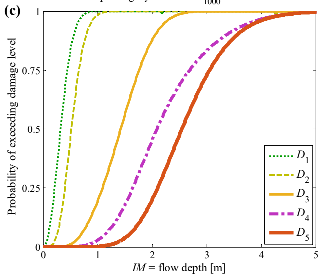
Sample fragility based on \theta_{1000} for Model 3
