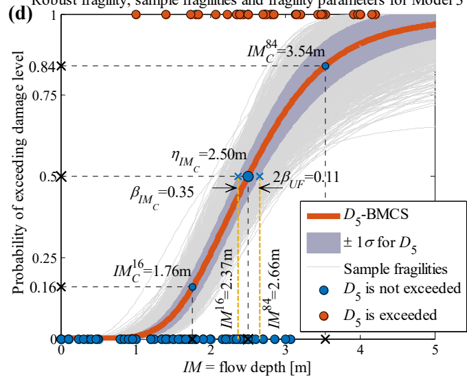
Robust fragility, sample fragilities and fragility parameters for Model 3
