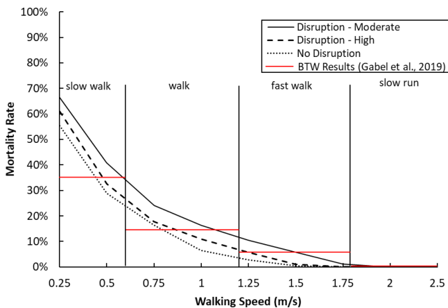
Figure 9. Network disruption impact: ABMS and BtW model result comparison.
