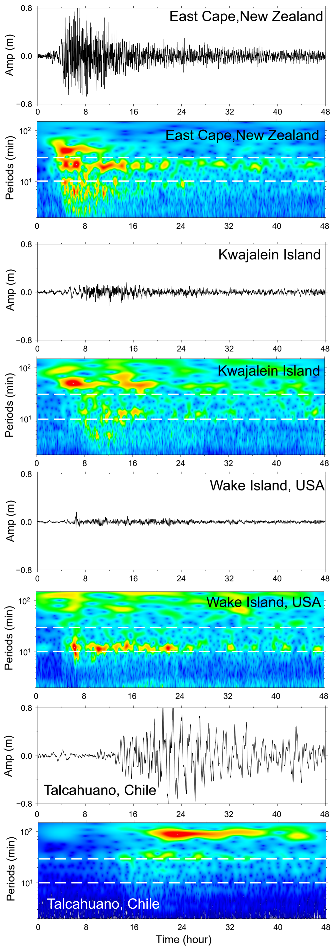
(a) the 2022 HTHH Tsunami
