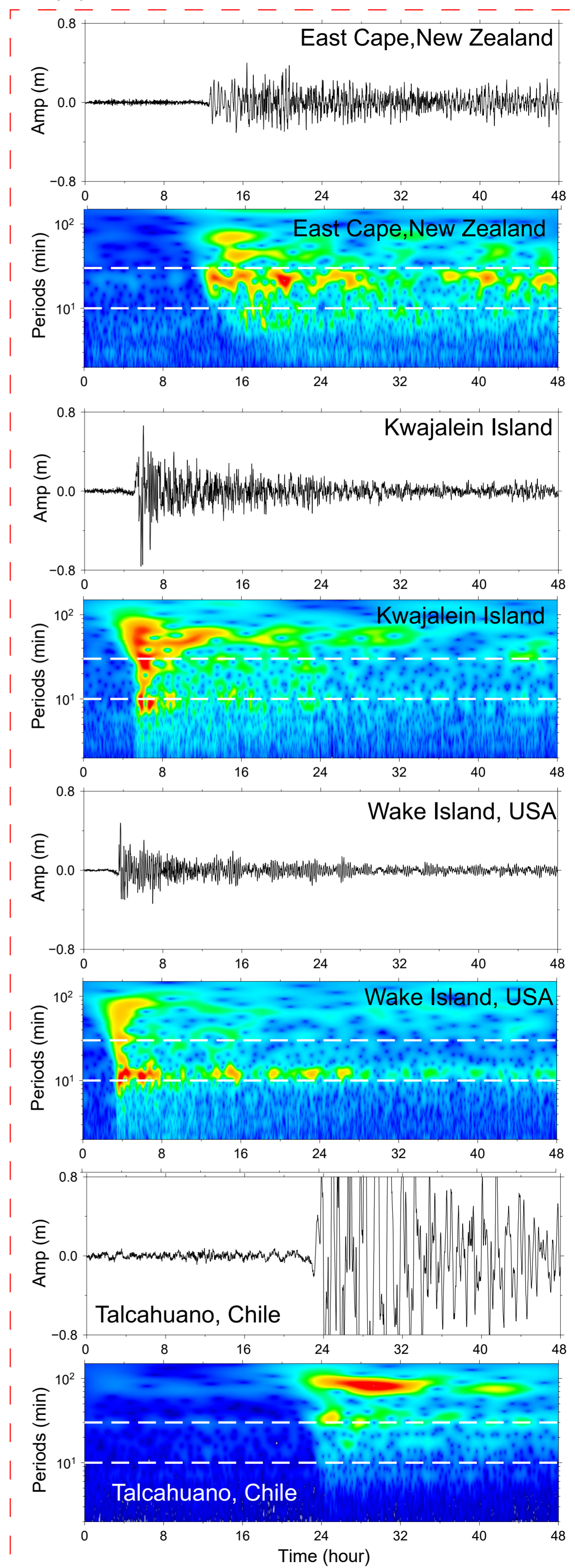
(b) the 2011 Tohoku Tsunami
