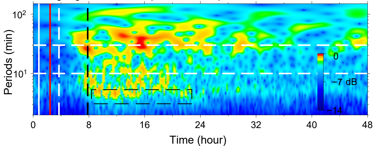
(b) Tide gauge: Charleston (New Zealand), 2680 km
