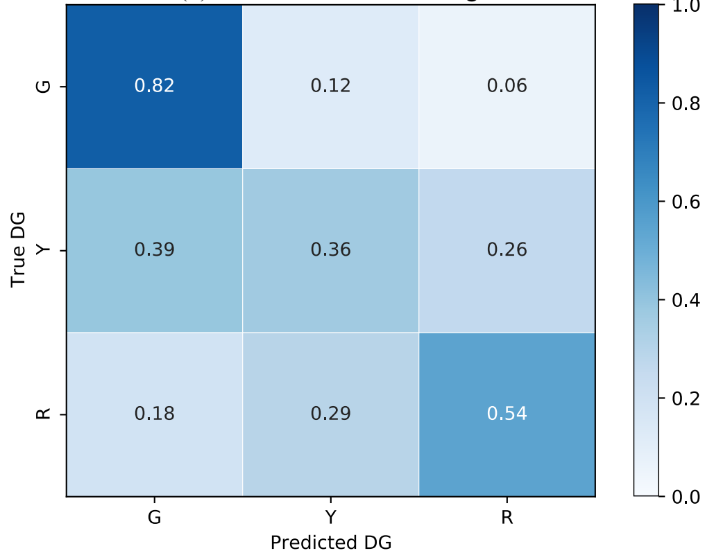
(b) TLS: full-features-setting
