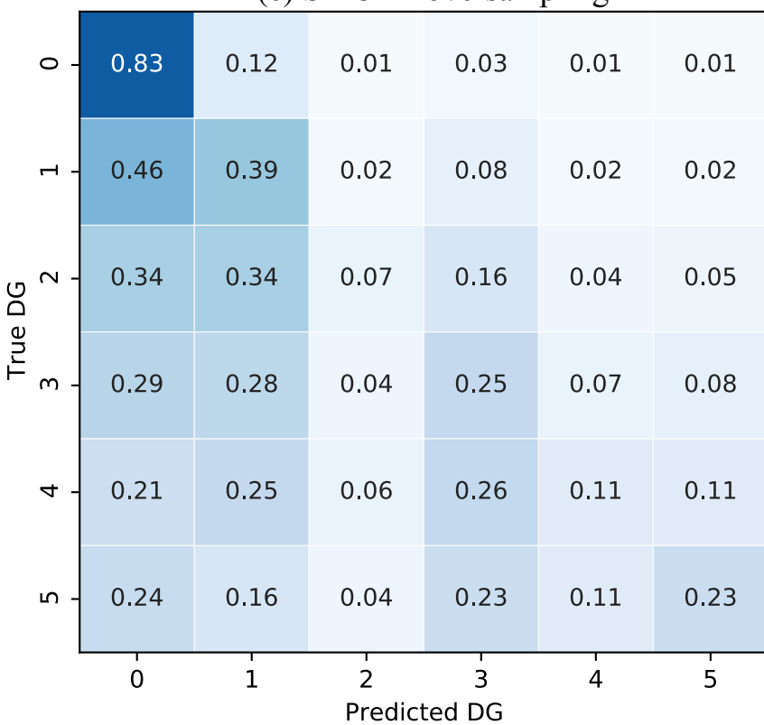
(c) SMOTE oversampling
