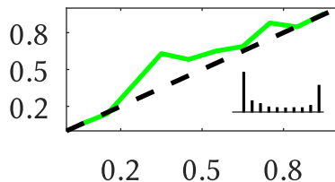
DenseNet
