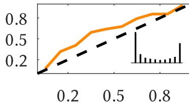
AlexNet
