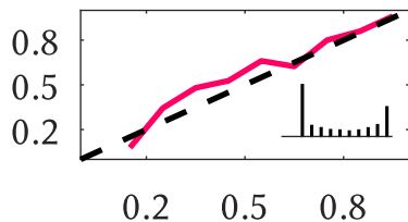
ALL-CNN
