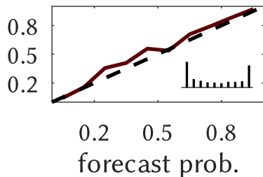
ALL-CNN
