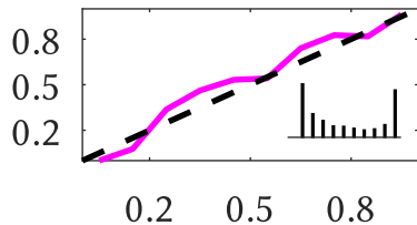
CIFAR-10
