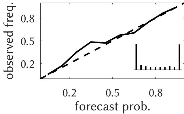
NNET
