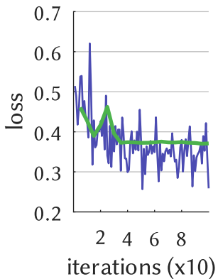
ALL-CNN
