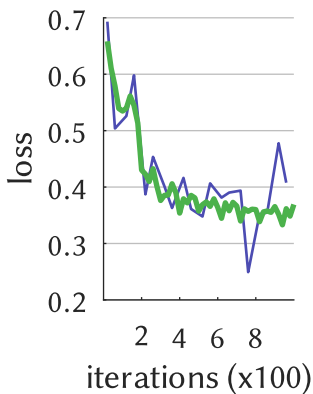
ALL-CNN
