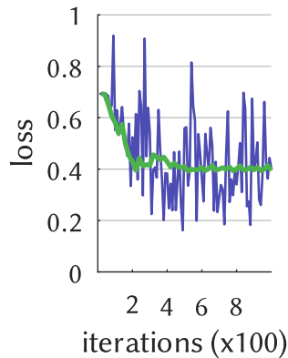
DenseNet
