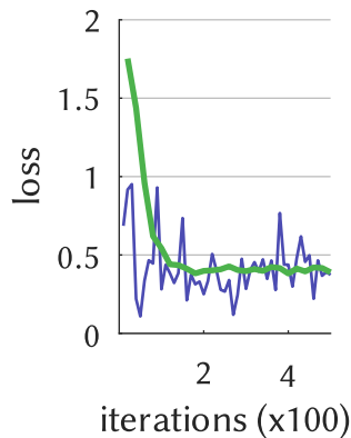
DenseNet
