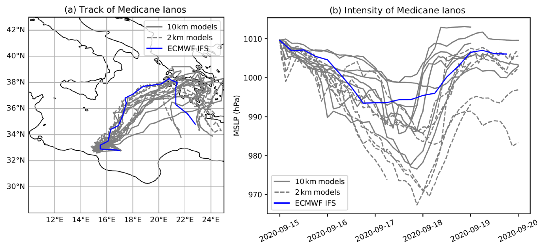
Figure 3. (a) Track (computed from the position of the minimum mean sea-level pressure) and (b) intensity (in terms of mean sea-level pressure) of Medcane Ianos as simulated by the different meteorological models.
