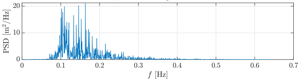
(c) Nonlinear continuous spectrum
